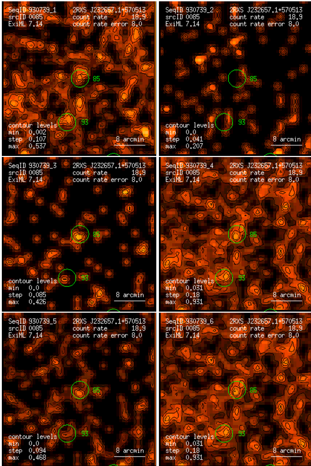
Figure 85: RASS 930739: detection 0085: band rate images, Gaussian filter: (1) PSPC channels 11 – 41, (2) 52 – 90, (3) 91 – 201, (4) 11 – 235, (5) 52 – 201, (6) 11 – 201. Broad band rates in counts/ks. Band rate contour levels in counts/ks/arcmin 2 .
