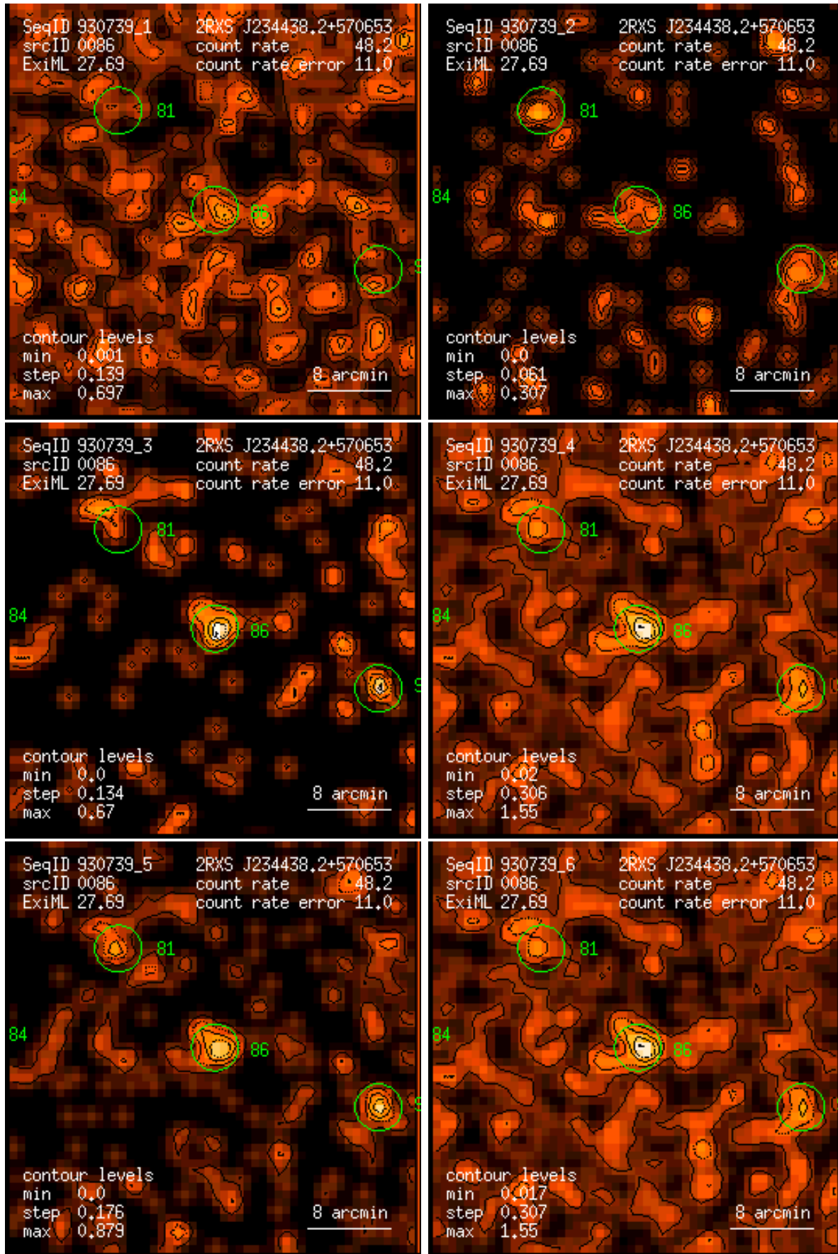
Figure 86: RASS 930739: detection 0086: band rate images, Gaussian filter: (1) PSPC channels 11 – 41, (2) 52 – 90, (3) 91 – 201, (4) 11 – 235, (5) 52 – 201, (6) 11 – 201. Broad band rates in counts/ks. Band rate contour levels in counts/ks/arcmin 2 .
