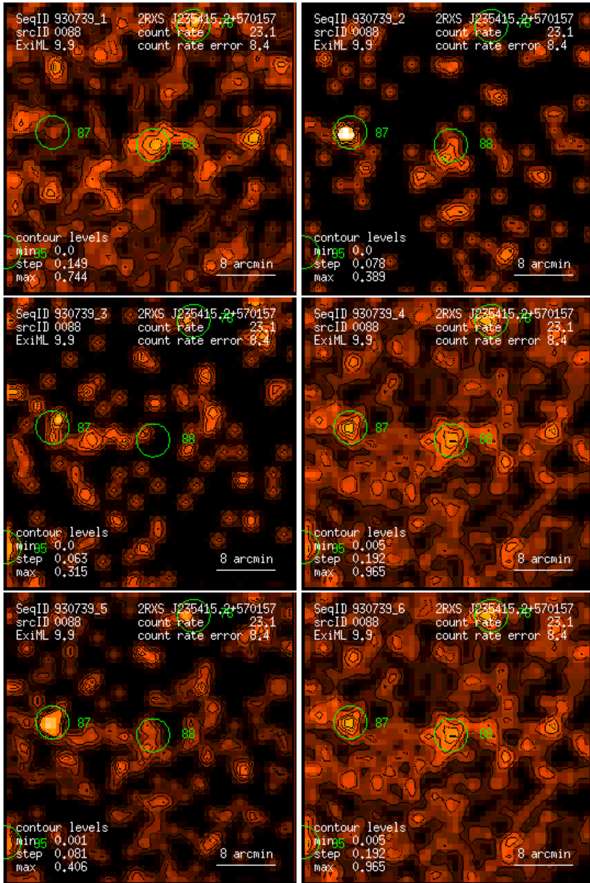
Figure 88: RASS 930739: detection 0088: band rate images, Gaussian filter: (1) PSPC channels 11 – 41, (2) 52 – 90, (3) 91 – 201, (4) 11 – 235, (5) 52 – 201, (6) 11 – 201. Broad band rates in counts/ks. Band rate contour levels in counts/ks/arcmin 2 .
