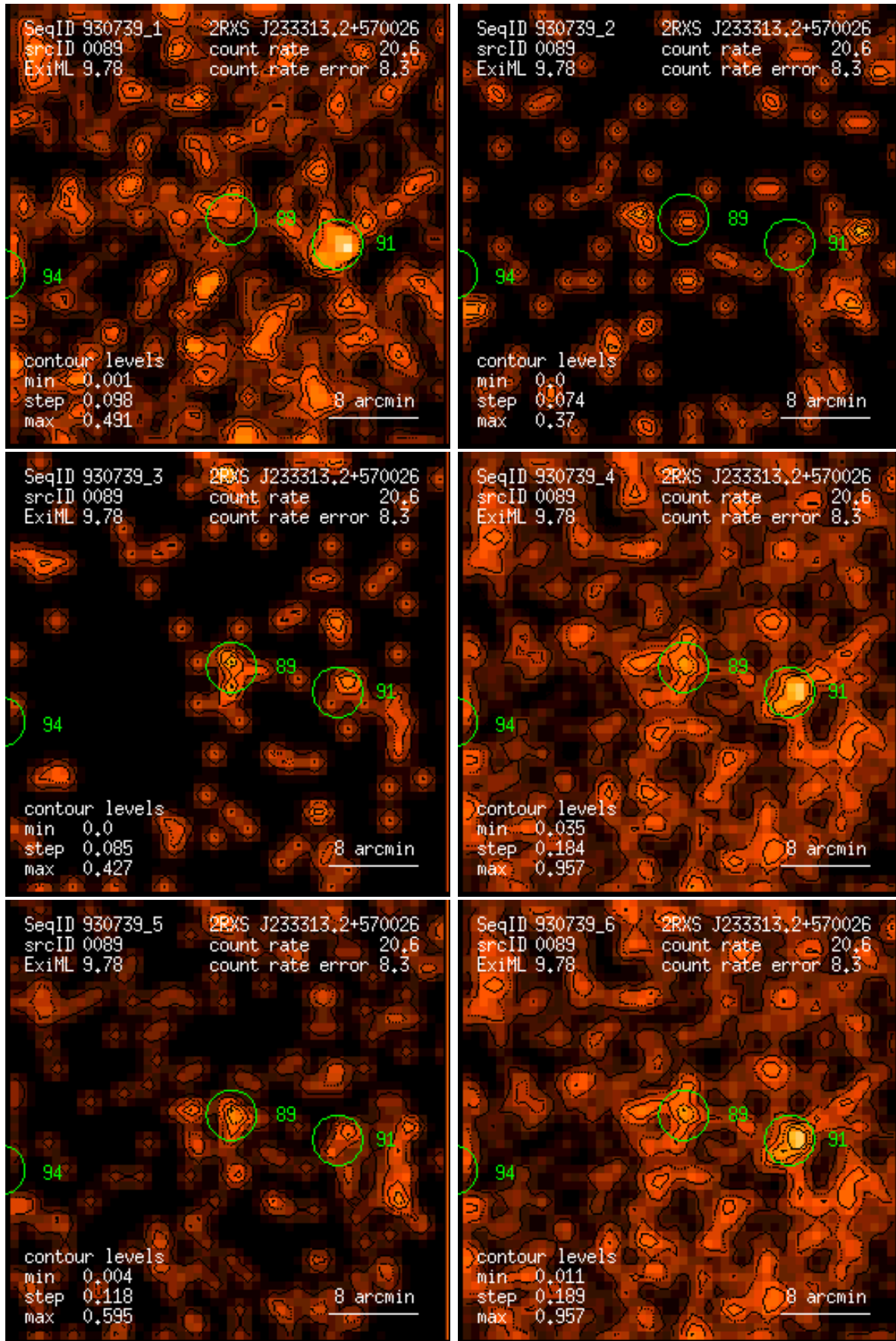
Figure 89: RASS 930739: detection 0089: band rate images, Gaussian filter: (1) PSPC channels 11 – 41, (2) 52 – 90, (3) 91 – 201, (4) 11 – 235, (5) 52 – 201, (6) 11 – 201. Broad band rates in counts/ks. Band rate contour levels in counts/ks/arcmin 2 .
