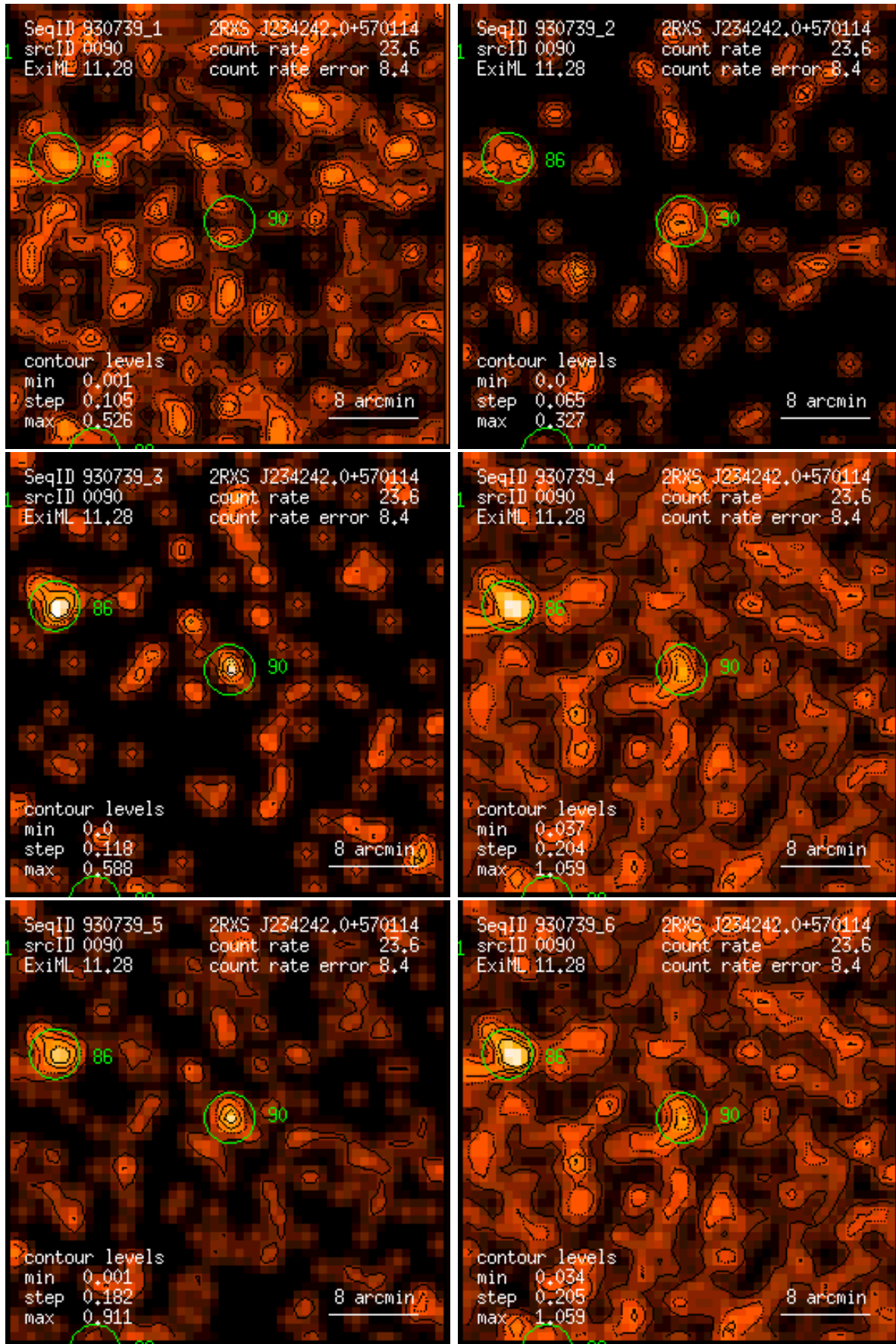
Figure 90: RASS 930739: detection 0090: band rate images, Gaussian filter: (1) PSPC channels 11 – 41, (2) 52 – 90, (3) 91 – 201, (4) 11 – 235, (5) 52 – 201, (6) 11 – 201. Broad band rates in counts/ks. Band rate contour levels in counts/ks/arcmin 2 .
