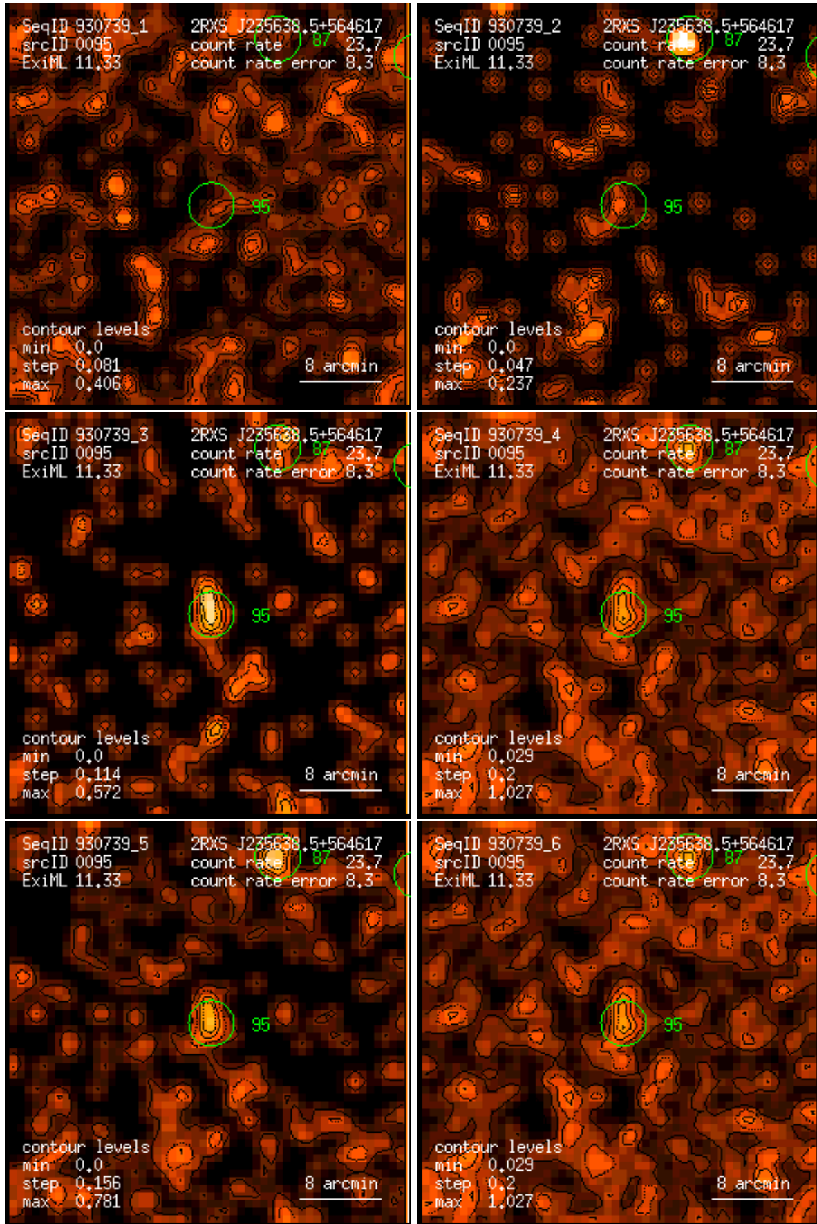
Figure 95: RASS 930739: detection 0095: band rate images, Gaussian filter: (1) PSPC channels 11 – 41, (2) 52 – 90, (3) 91 – 201, (4) 11 – 235, (5) 52 – 201, (6) 11 – 201. Broad band rates in counts/ks. Band rate contour levels in counts/ks/arcmin 2 .
