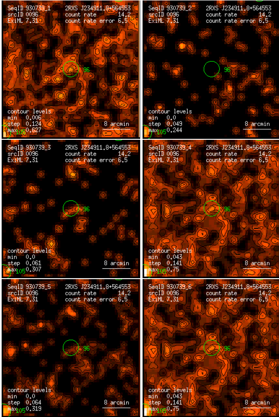
Figure 96: RASS 930739: detection 0096: band rate images, Gaussian filter: (1) PSPC channels 11 – 41, (2) 52 – 90, (3) 91 – 201, (4) 11 – 235, (5) 52 – 201, (6) 11 – 201. Broad band rates in counts/ks. Band rate contour levels in counts/ks/arcmin 2 .
