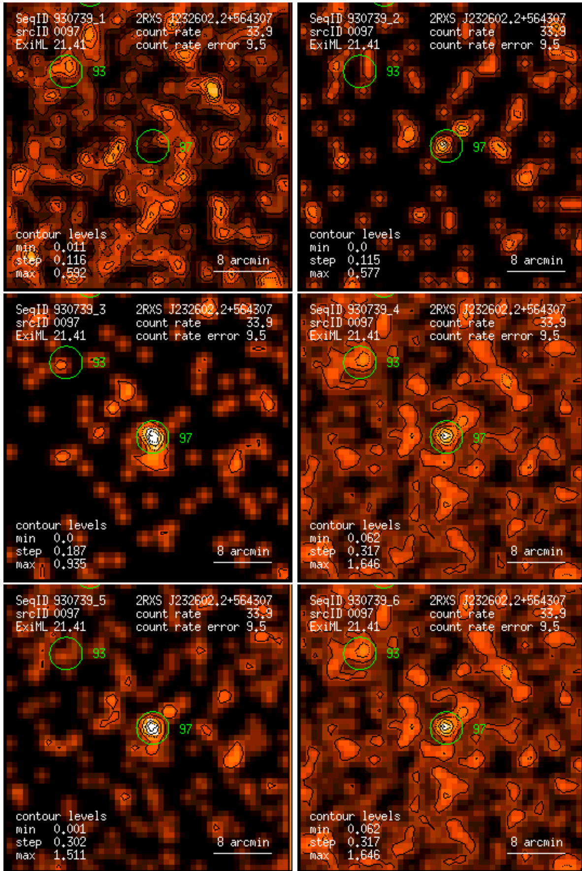
Figure 97: RASS 930739: detection 0097: band rate images, Gaussian filter: (1) PSPC channels 11 – 41, (2) 52 – 90, (3) 91 – 201, (4) 11 – 235, (5) 52 – 201, (6) 11 – 201. Broad band rates in counts/ks. Band rate contour levels in counts/ks/arcmin 2 .
