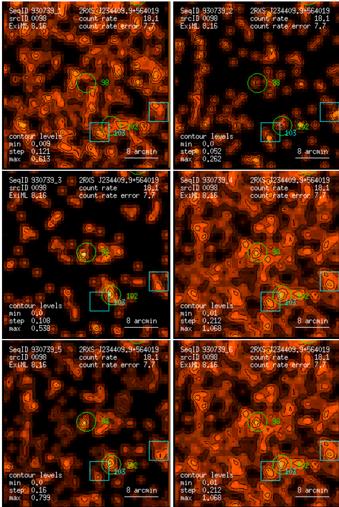
Figure 98: RASS 930739: detection 0098: band rate images, Gaussian filter: (1) PSPC channels 11 – 41, (2) 52 – 90, (3) 91 – 201, (4) 11 – 235, (5) 52 – 201, (6) 11 – 201. Broad band rates in counts/ks. Band rate contour levels in counts/ks/arcmin 2 .
