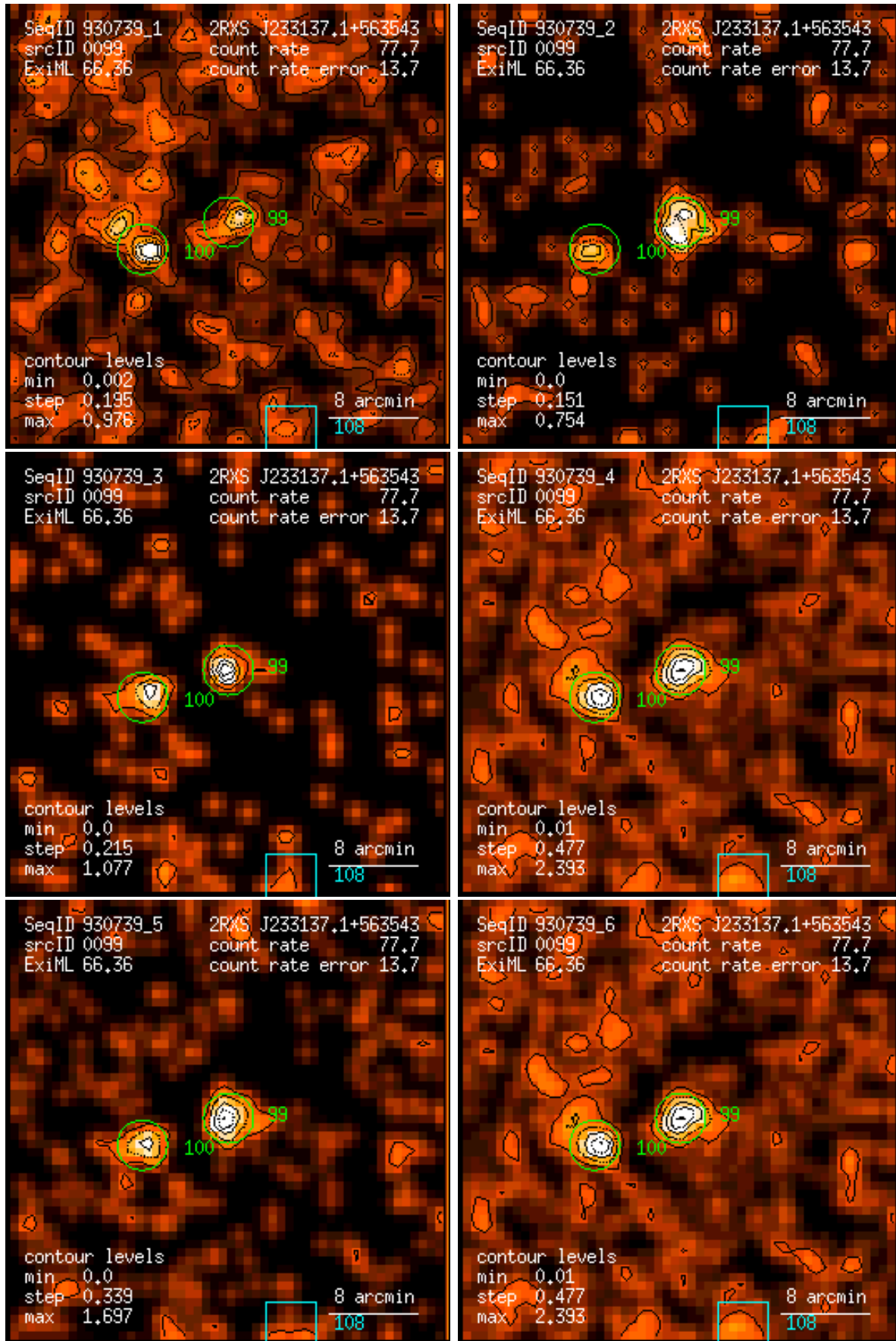
Figure 99: RASS 930739: detection 0099: band rate images, Gaussian filter: (1) PSPC channels 11 – 41, (2) 52 – 90, (3) 91 – 201, (4) 11 – 235, (5) 52 – 201, (6) 11 – 201. Broad band rates in counts/ks. Band rate contour levels in counts/ks/arcmin 2 .
