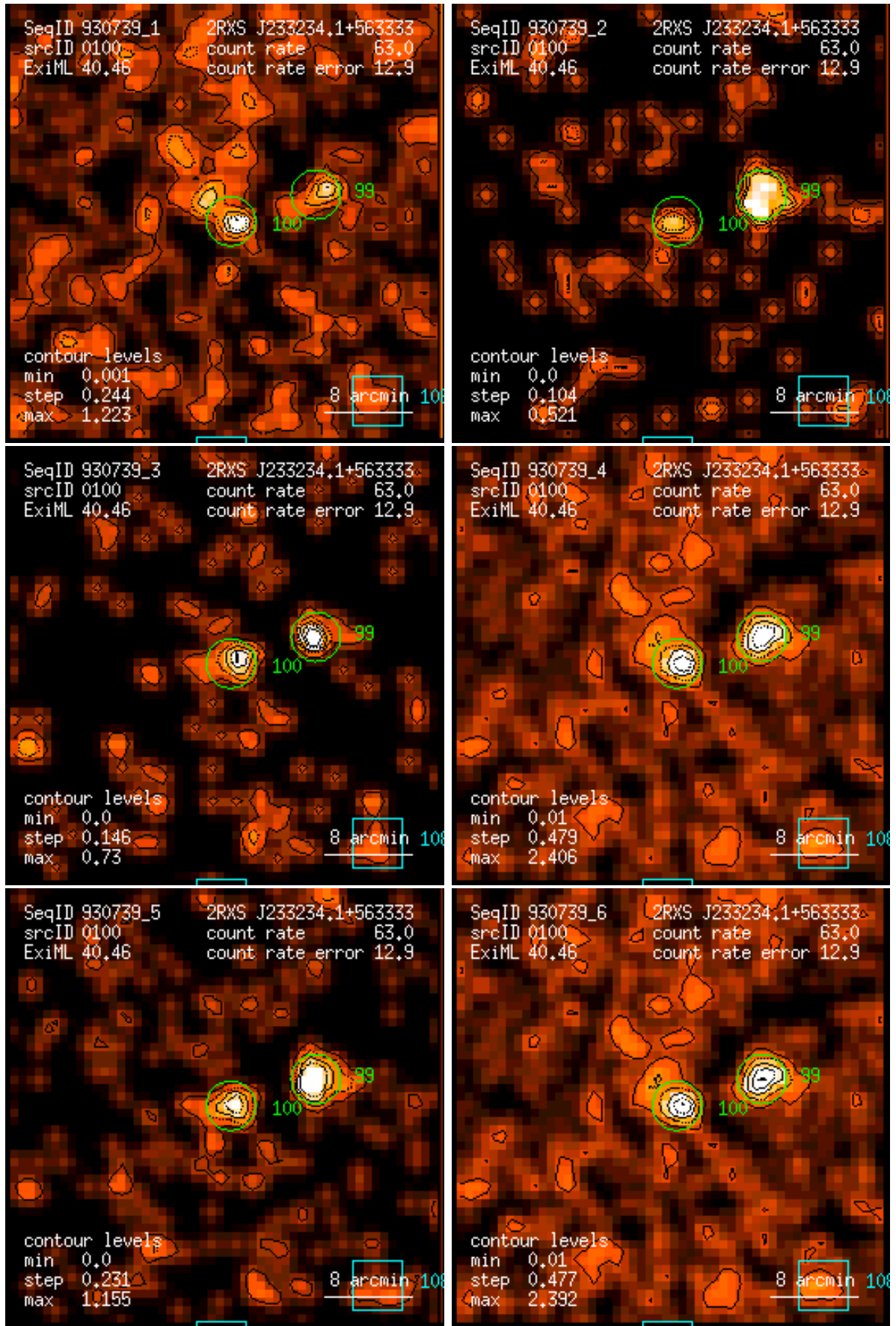
Figure 100: RASS 930739: detection 0100: band rate images, Gaussian filter: (1) PSPC channels 11 – 41, (2) 52 – 90, (3) 91 – 201, (4) 11 – 235, (5) 52 – 201, (6) 11 – 201. Broad band rates in counts/ks. Band rate contour levels in counts/ks/arcmin 2 .
