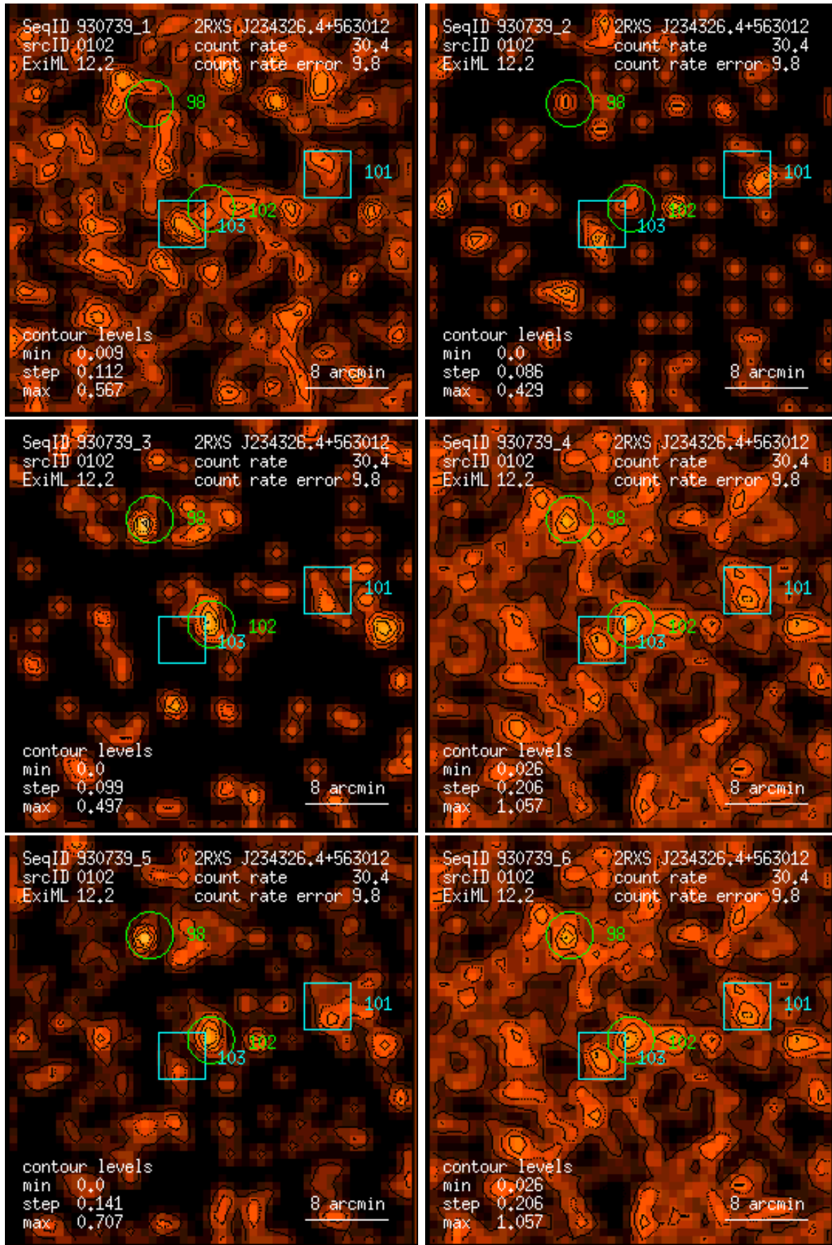
Figure 102: RASS 930739: detection 0102: band rate images, Gaussian filter: (1) PSPC channels 11 – 41, (2) 52 – 90, (3) 91 – 201, (4) 11 – 235, (5) 52 – 201, (6) 11 – 201. Broad band rates in counts/ks. Band rate contour levels in counts/ks/arcmin 2 .
