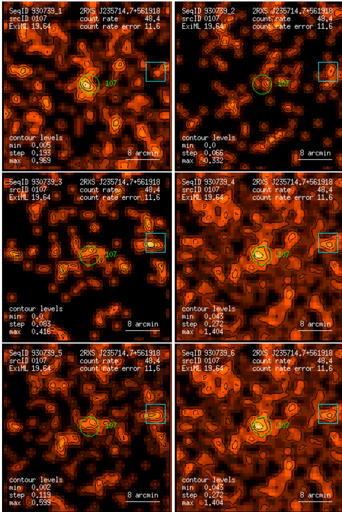
Figure 107: RASS 930739: detection 0107: band rate images, Gaussian filter: (1) PSPC channels 11 – 41, (2) 52 – 90, (3) 91 – 201, (4) 11 – 235, (5) 52 – 201, (6) 11 – 201. Broad band rates in counts/ks. Band rate contour levels in counts/ks/arcmin 2 .
