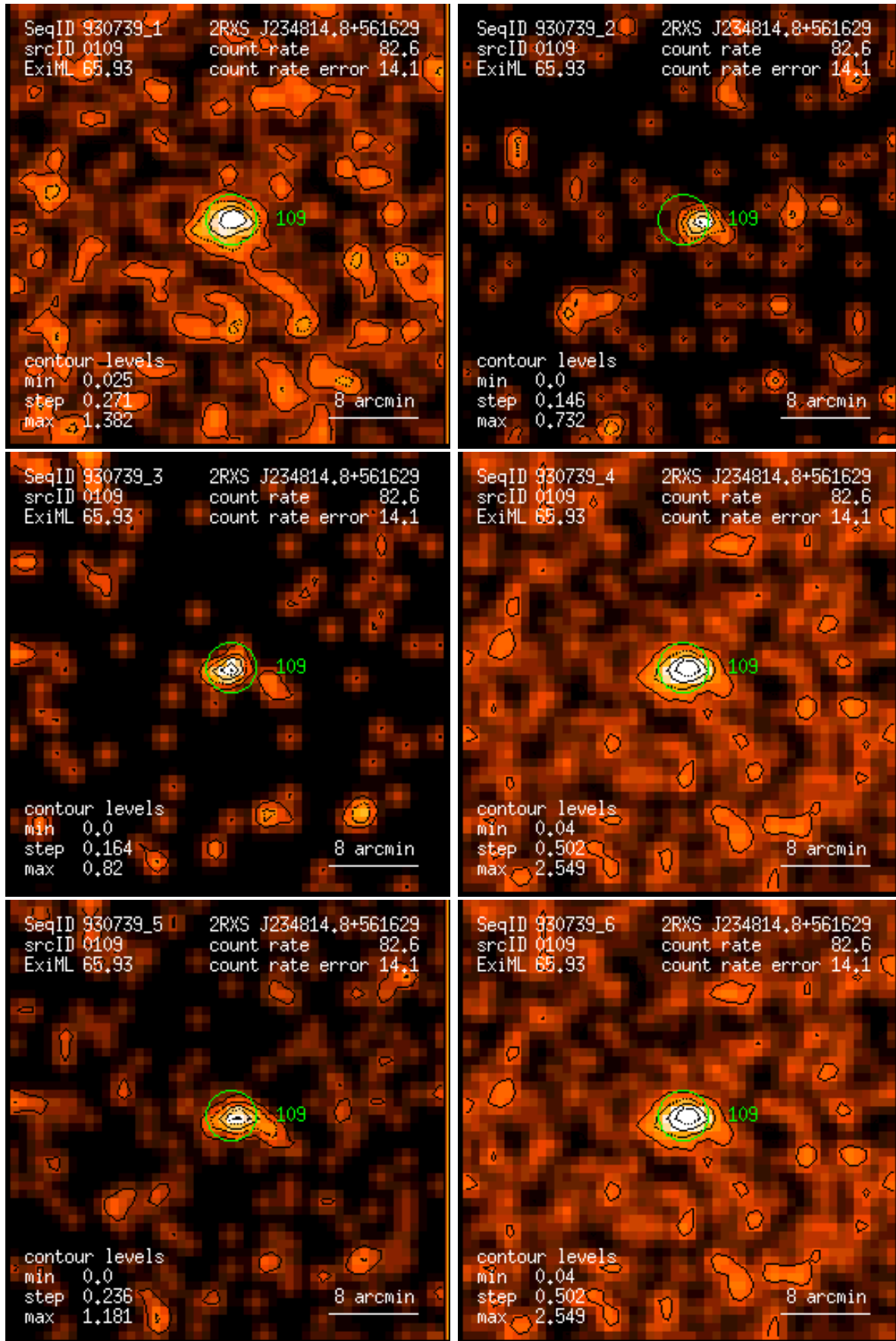
Figure 109: RASS 930739: detection 0109: band rate images, Gaussian filter: (1) PSPC channels 11 – 41, (2) 52 – 90, (3) 91 – 201, (4) 11 – 235, (5) 52 – 201, (6) 11 – 201. Broad band rates in counts/ks. Band rate contour levels in counts/ks/arcmin 2 .
