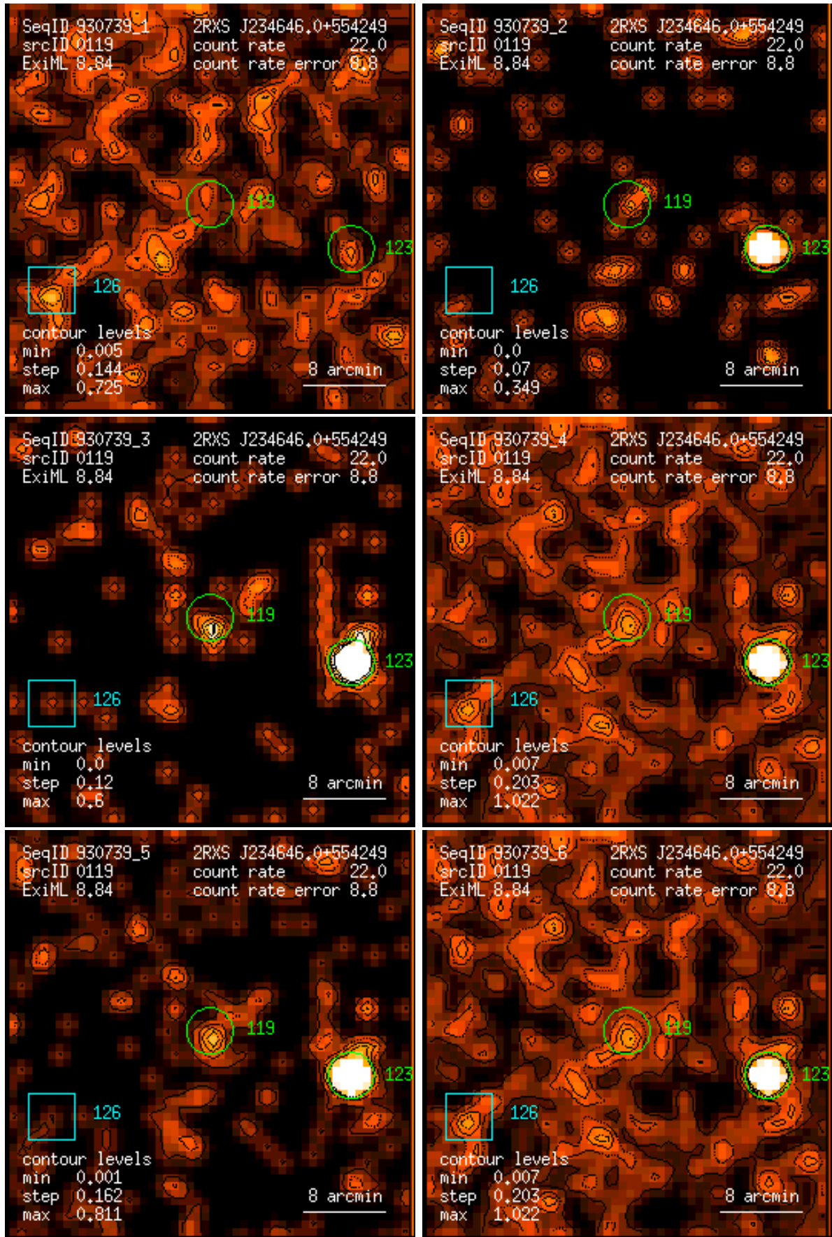
Figure 119: RASS 930739: detection 0119: band rate images, Gaussian filter: (1) PSPC channels 11 – 41, (2) 52 – 90, (3) 91 – 201, (4) 11 – 235, (5) 52 – 201, (6) 11 – 201. Broad band rates in counts/ks. Band rate contour levels in counts/ks/arcmin 2 .
