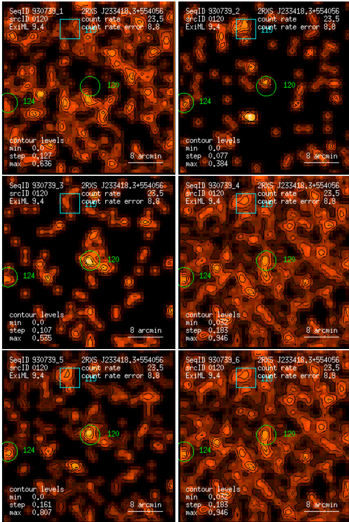
Figure 120: RASS 930739: detection 0120: band rate images, Gaussian filter: (1) PSPC channels 11 – 41, (2) 52 – 90, (3) 91 – 201, (4) 11 – 235, (5) 52 – 201, (6) 11 – 201. Broad band rates in counts/ks. Band rate contour levels in counts/ks/arcmin 2 .
