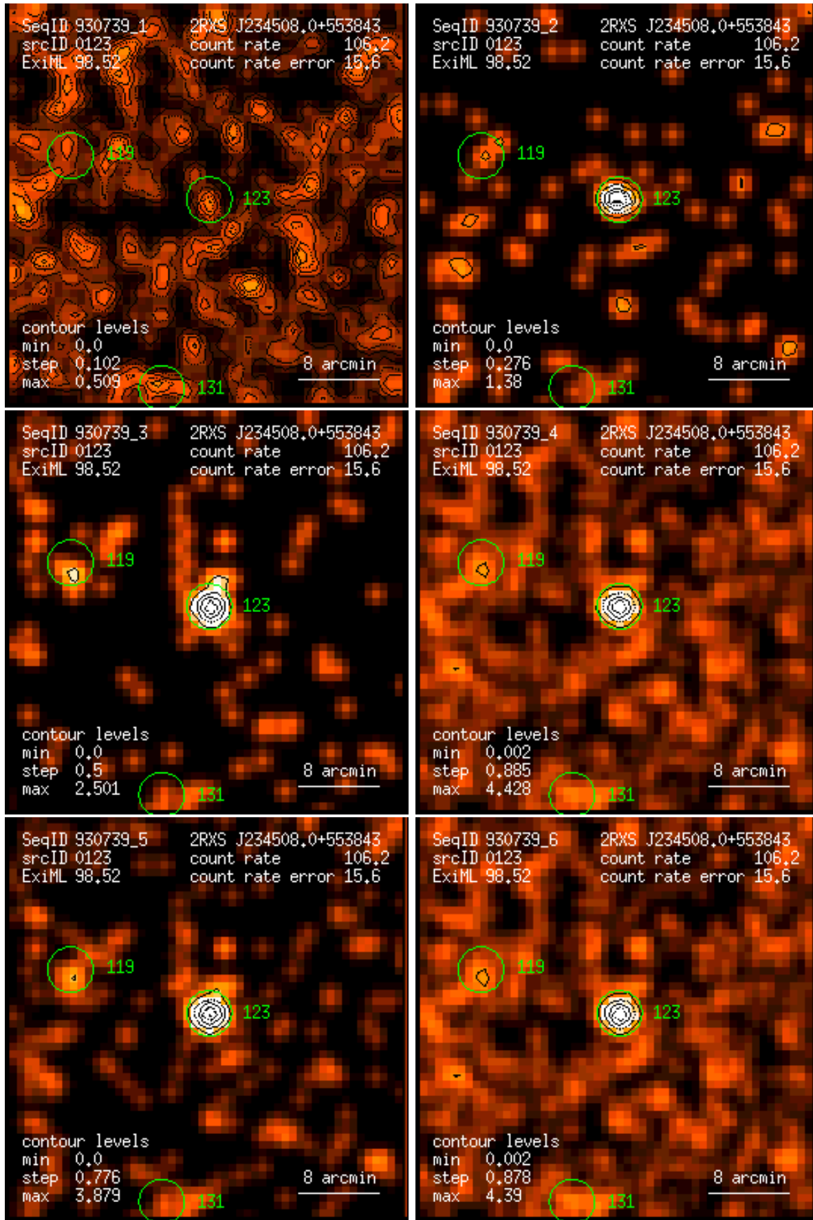
Figure 123: RASS 930739: detection 0123: band rate images, Gaussian filter: (1) PSPC channels 11 – 41, (2) 52 – 90, (3) 91 – 201, (4) 11 – 235, (5) 52 – 201, (6) 11 – 201. Broad band rates in counts/ks. Band rate contour levels in counts/ks/arcmin 2 .
