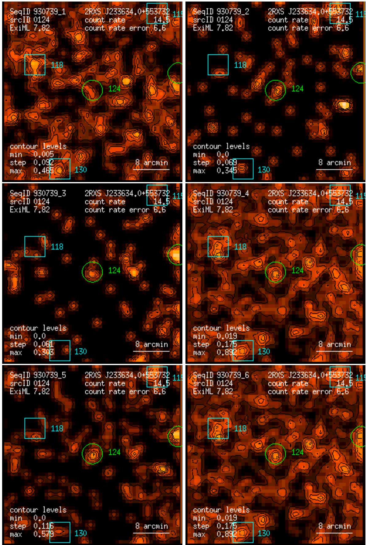
Figure 124: RASS 930739: detection 0124: band rate images, Gaussian filter: (1) PSPC channels 11 – 41, (2) 52 – 90, (3) 91 – 201, (4) 11 – 235, (5) 52 – 201, (6) 11 – 201. Broad band rates in counts/ks. Band rate contour levels in counts/ks/arcmin 2 .
