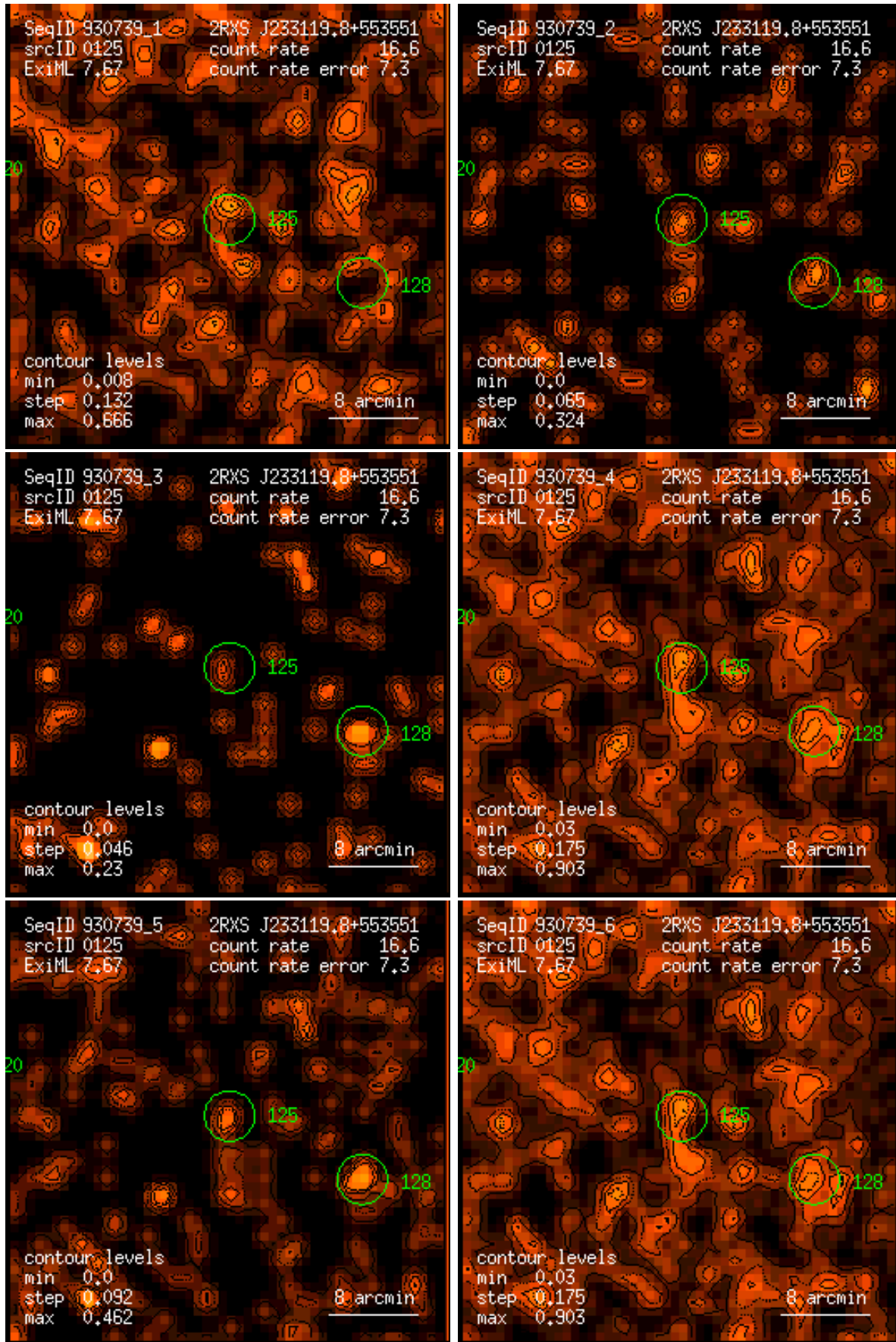
Figure 125: RASS 930739: detection 0125: band rate images, Gaussian filter: (1) PSPC channels 11 – 41, (2) 52 – 90, (3) 91 – 201, (4) 11 – 235, (5) 52 – 201, (6) 11 – 201. Broad band rates in counts/ks. Band rate contour levels in counts/ks/arcmin 2 .
