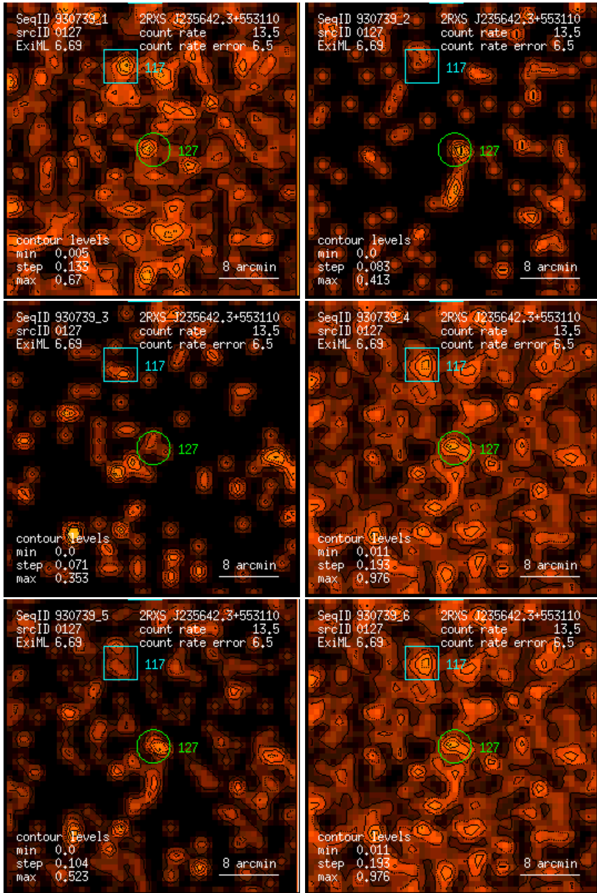
Figure 127: RASS 930739: detection 0127: band rate images, Gaussian filter: (1) PSPC channels 11 – 41, (2) 52 – 90, (3) 91 – 201, (4) 11 – 235, (5) 52 – 201, (6) 11 – 201. Broad band rates in counts/ks. Band rate contour levels in counts/ks/arcmin 2 .
