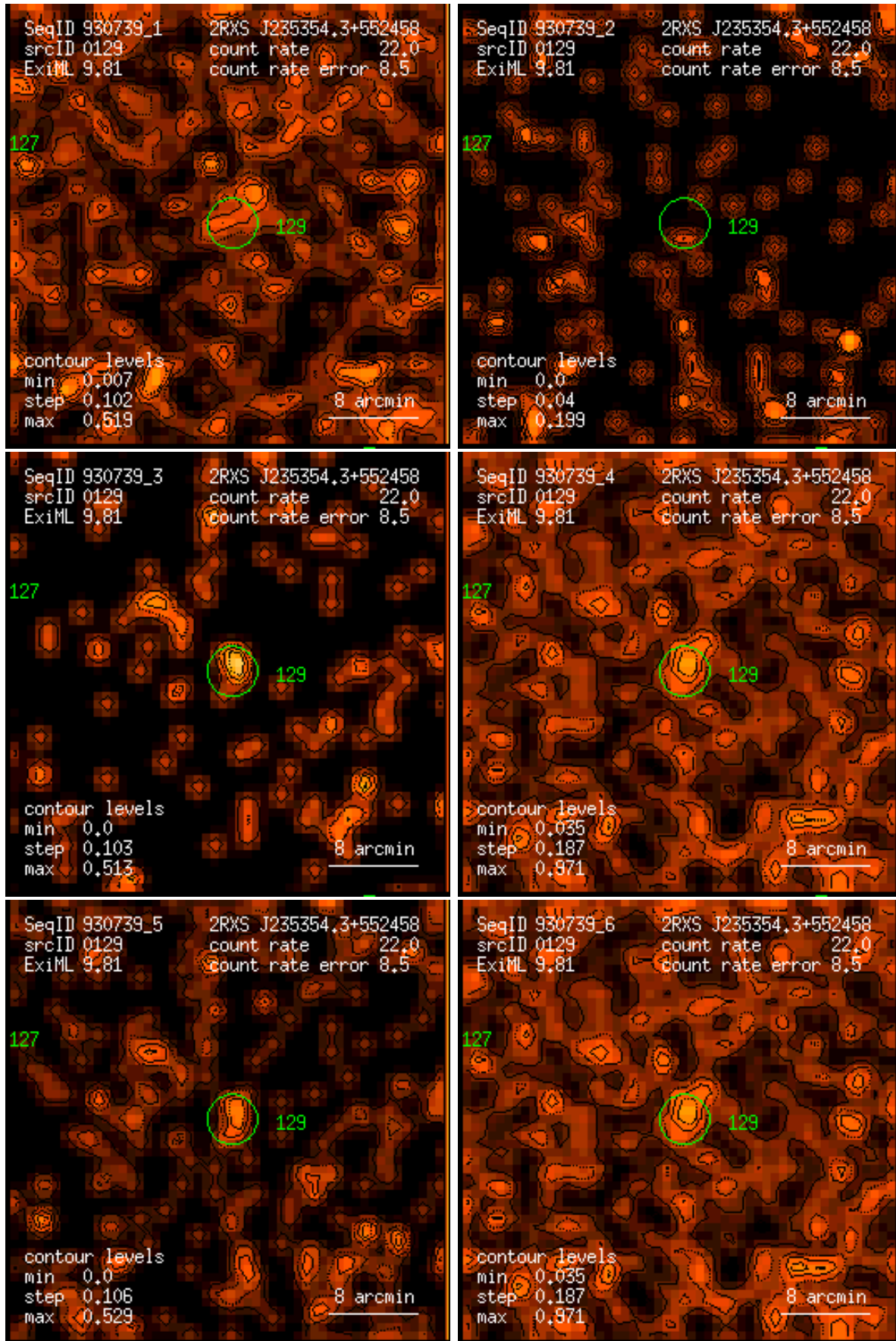
Figure 129: RASS 930739: detection 0129: band rate images, Gaussian filter: (1) PSPC channels 11 – 41, (2) 52 – 90, (3) 91 – 201, (4) 11 – 235, (5) 52 – 201, (6) 11 – 201. Broad band rates in counts/ks. Band rate contour levels in counts/ks/arcmin 2 .
