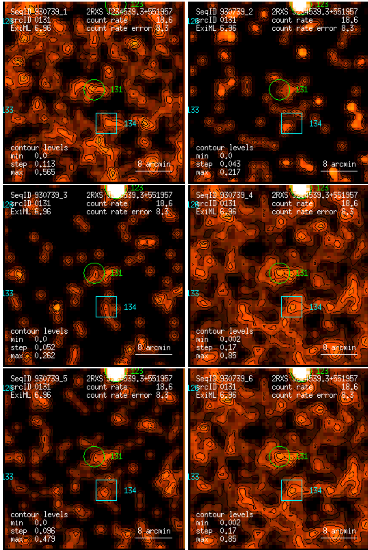
Figure 131: RASS 930739: detection 0131: band rate images, Gaussian filter: (1) PSPC channels 11 – 41, (2) 52 – 90, (3) 91 – 201, (4) 11 – 235, (5) 52 – 201, (6) 11 – 201. Broad band rates in counts/ks. Band rate contour levels in counts/ks/arcmin 2 .
