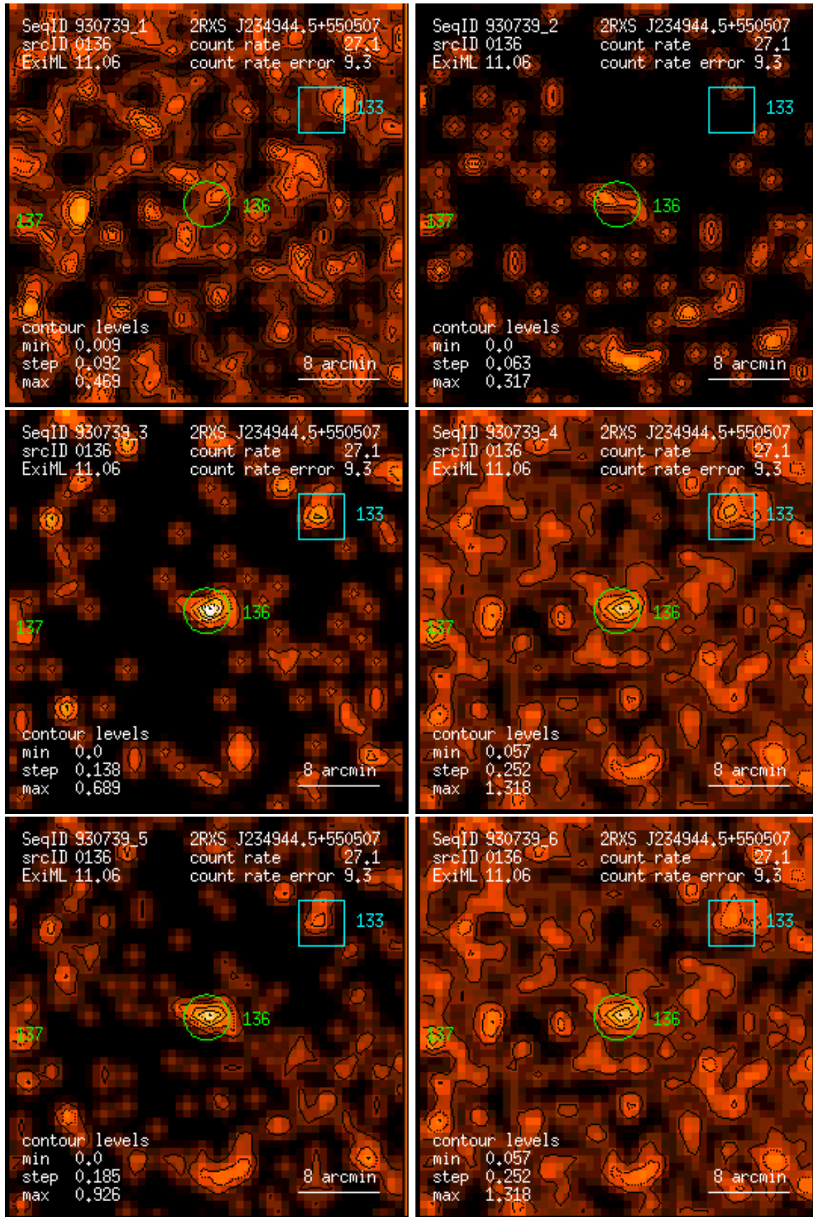
Figure 136: RASS 930739: detection 0136: band rate images, Gaussian filter: (1) PSPC channels 11 – 41, (2) 52 – 90, (3) 91 – 201, (4) 11 – 235, (5) 52 – 201, (6) 11 – 201. Broad band rates in counts/ks. Band rate contour levels in counts/ks/arcmin 2 .
