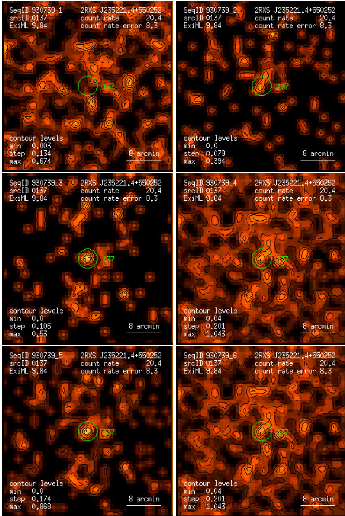
Figure 137: RASS 930739: detection 0137: band rate images, Gaussian filter: (1) PSPC channels 11 – 41, (2) 52 – 90, (3) 91 – 201, (4) 11 – 235, (5) 52 – 201, (6) 11 – 201. Broad band rates in counts/ks. Band rate contour levels in counts/ks/arcmin 2 .
