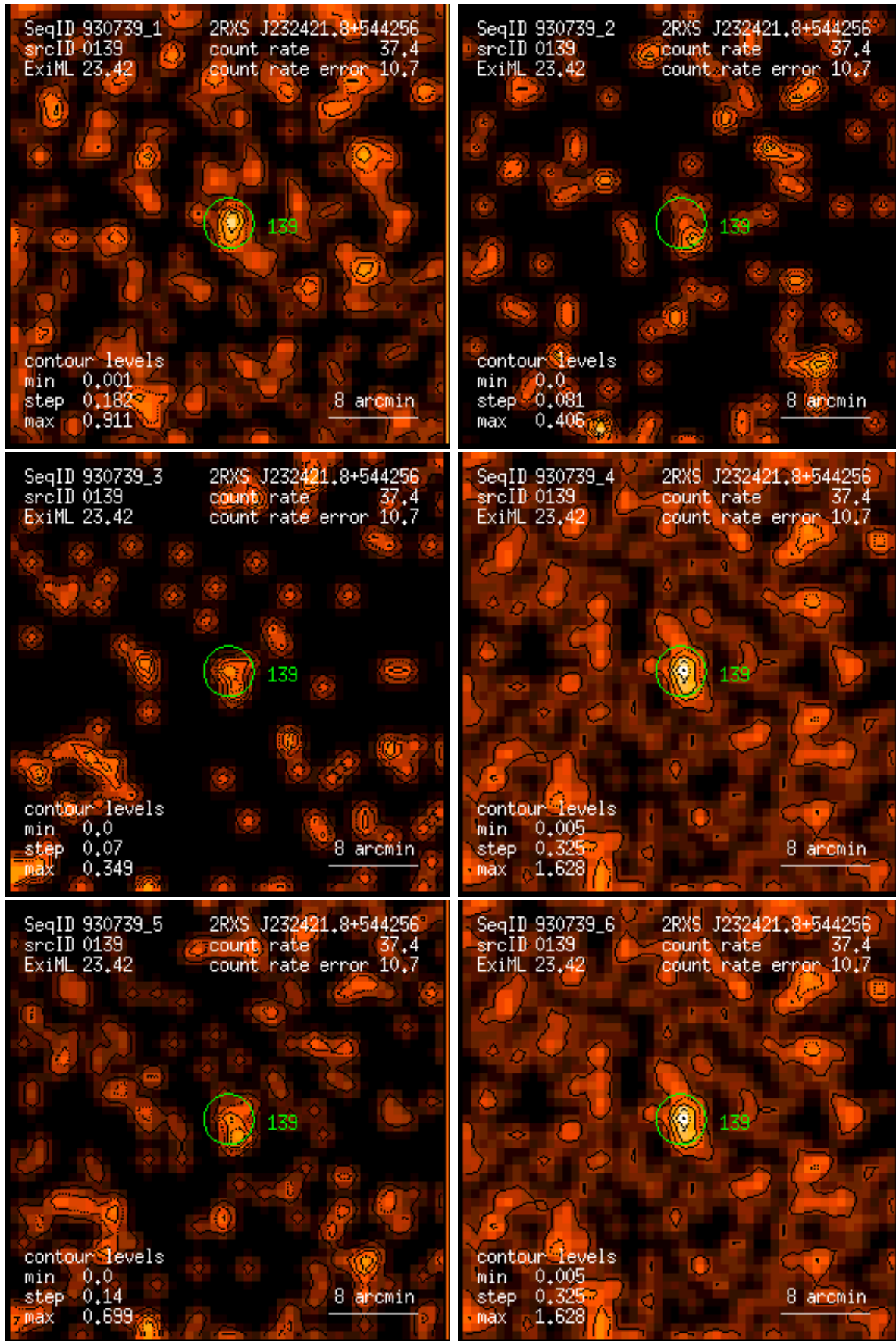
Figure 139: RASS 930739: detection 0139: band rate images, Gaussian filter: (1) PSPC channels 11 – 41, (2) 52 – 90, (3) 91 – 201, (4) 11 – 235, (5) 52 – 201, (6) 11 – 201. Broad band rates in counts/ks. Band rate contour levels in counts/ks/arcmin 2 .
