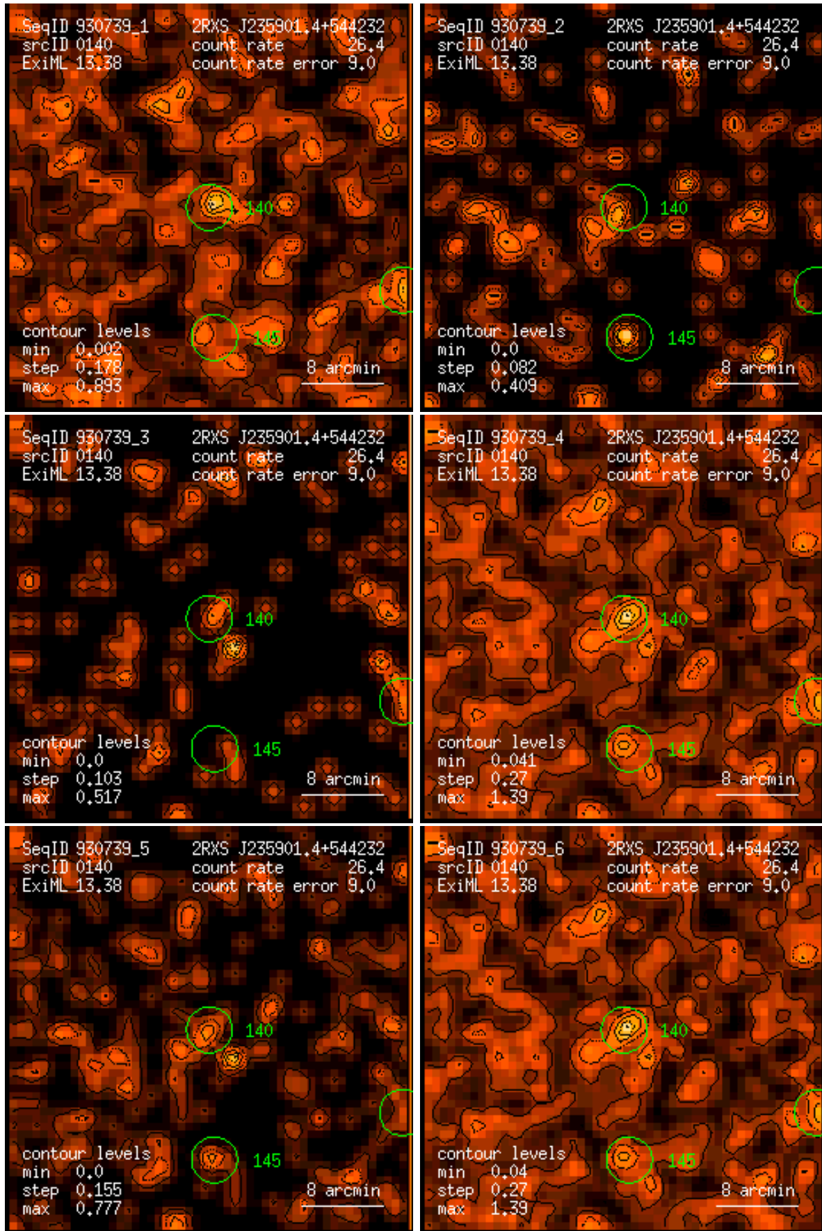
Figure 140: RASS 930739: detection 0140: band rate images, Gaussian filter: (1) PSPC channels 11 – 41, (2) 52 – 90, (3) 91 – 201, (4) 11 – 235, (5) 52 – 201, (6) 11 – 201. Broad band rates in counts/ks. Band rate contour levels in counts/ks/arcmin 2 .
