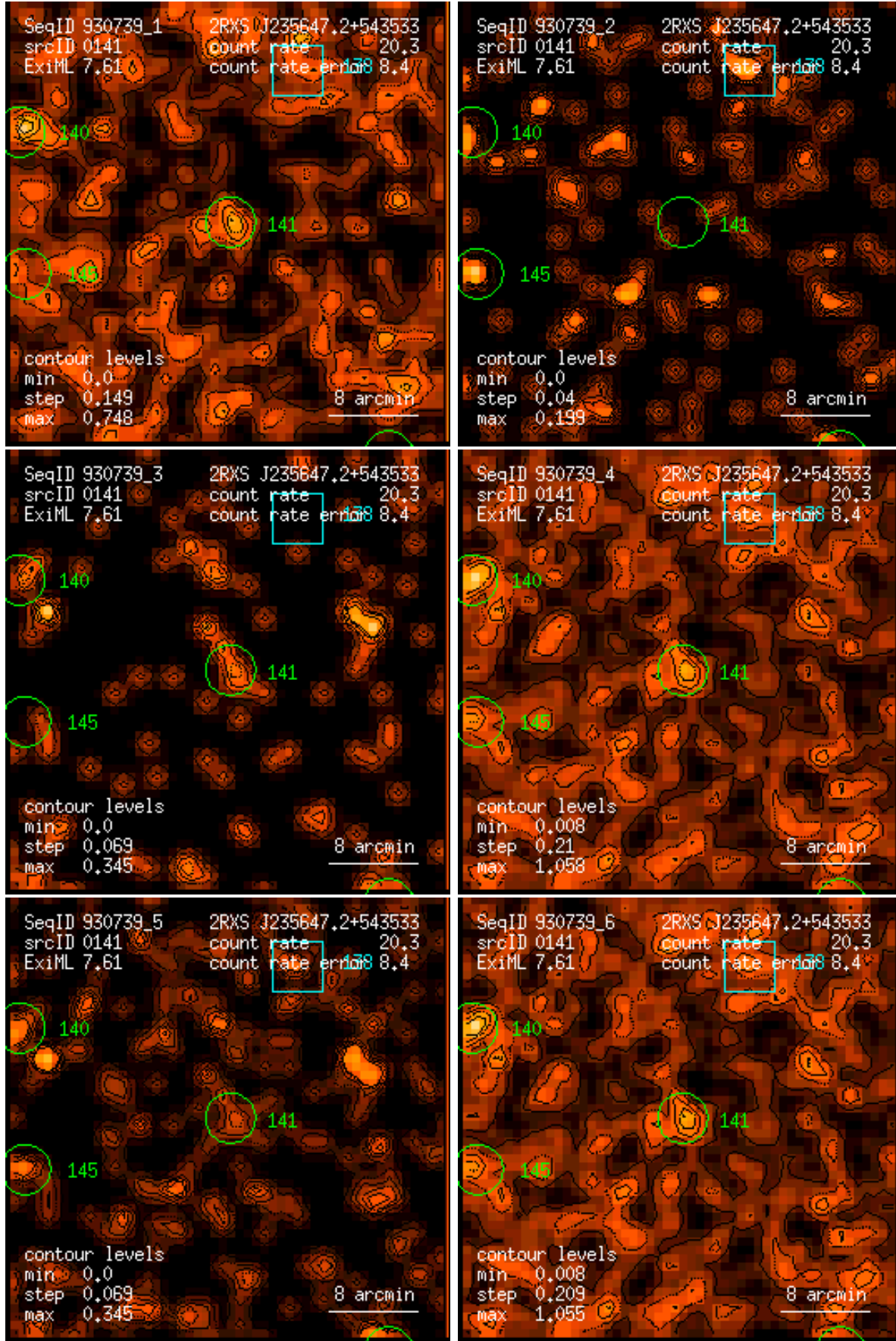
Figure 141: RASS 930739: detection 0141: band rate images, Gaussian filter: (1) PSPC channels 11 – 41, (2) 52 – 90, (3) 91 – 201, (4) 11 – 235, (5) 52 – 201, (6) 11 – 201. Broad band rates in counts/ks. Band rate contour levels in counts/ks/arcmin 2 .
