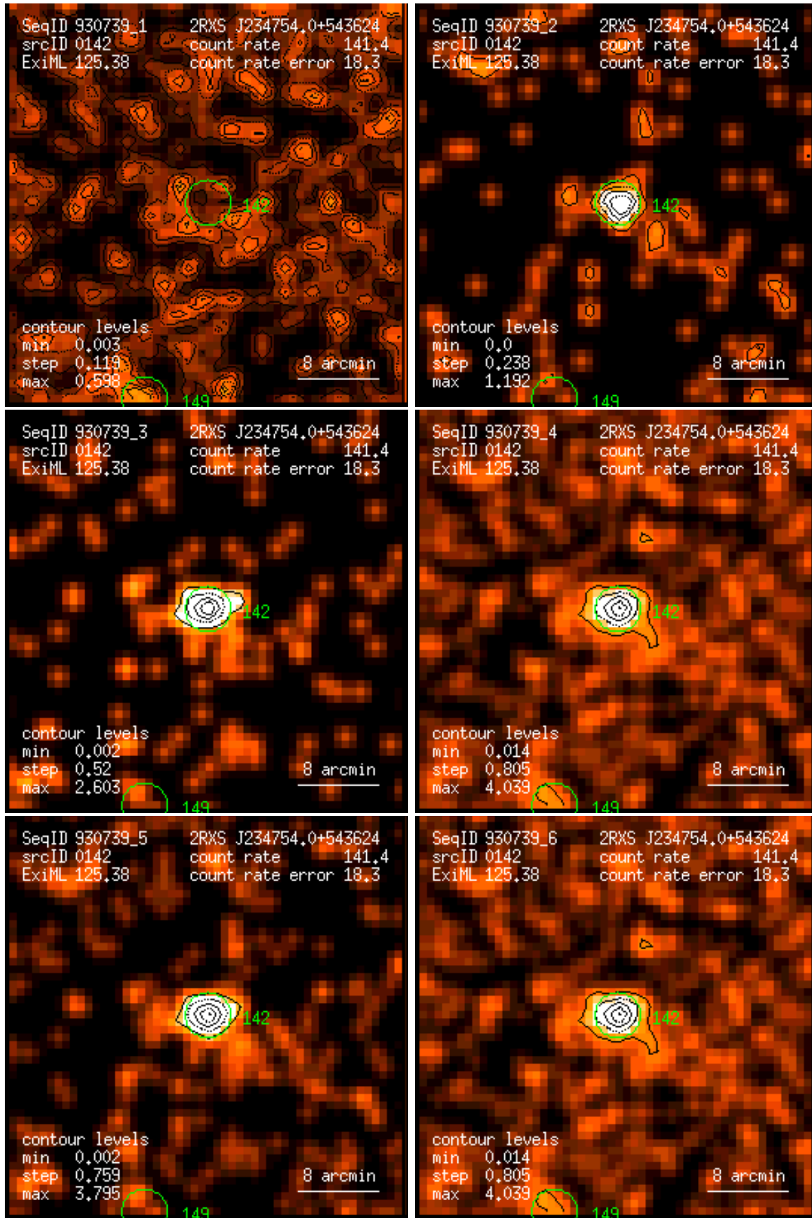
Figure 142: RASS 930739: detection 0142: band rate images, Gaussian filter: (1) PSPC channels 11 – 41, (2) 52 – 90, (3) 91 – 201, (4) 11 – 235, (5) 52 – 201, (6) 11 – 201. Broad band rates in counts/ks. Band rate contour levels in counts/ks/arcmin 2 .
