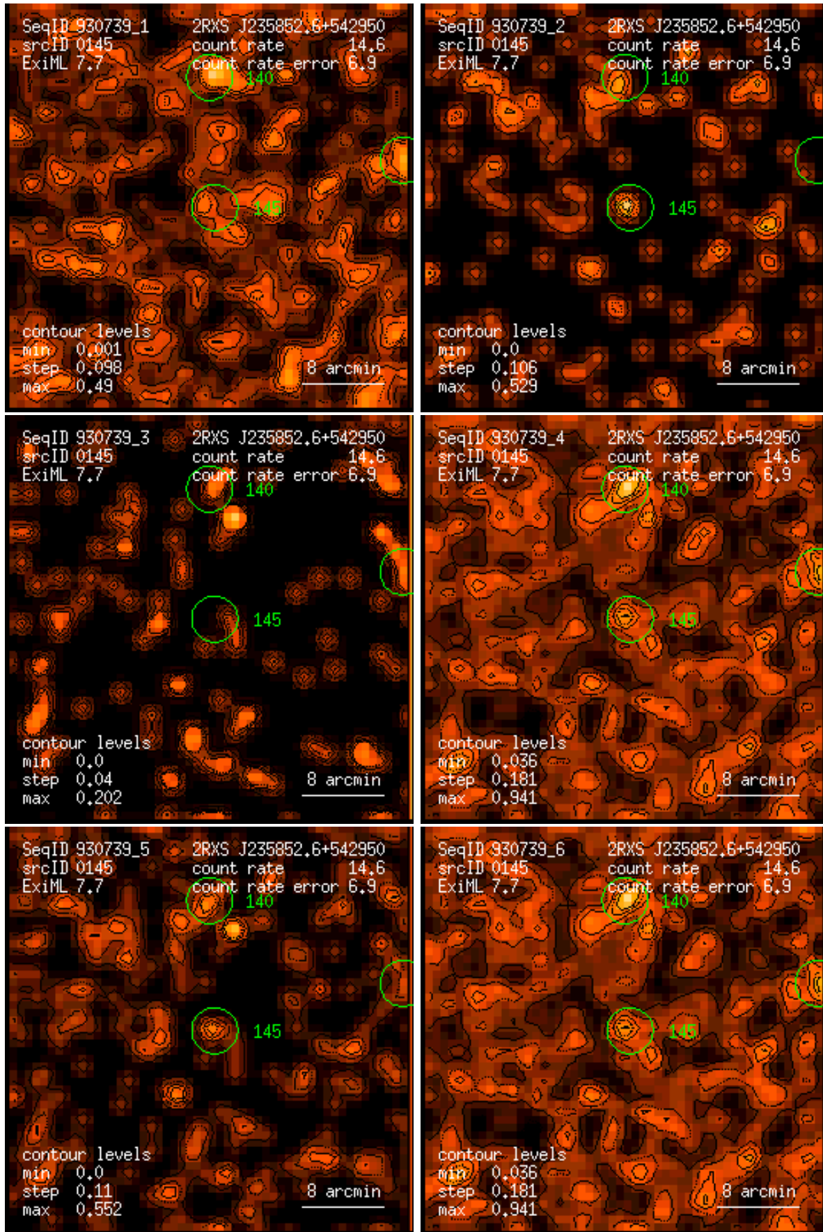
Figure 145: RASS 930739: detection 0145: band rate images, Gaussian filter: (1) PSPC channels 11 – 41, (2) 52 – 90, (3) 91 – 201, (4) 11 – 235, (5) 52 – 201, (6) 11 – 201. Broad band rates in counts/ks. Band rate contour levels in counts/ks/arcmin 2 .
