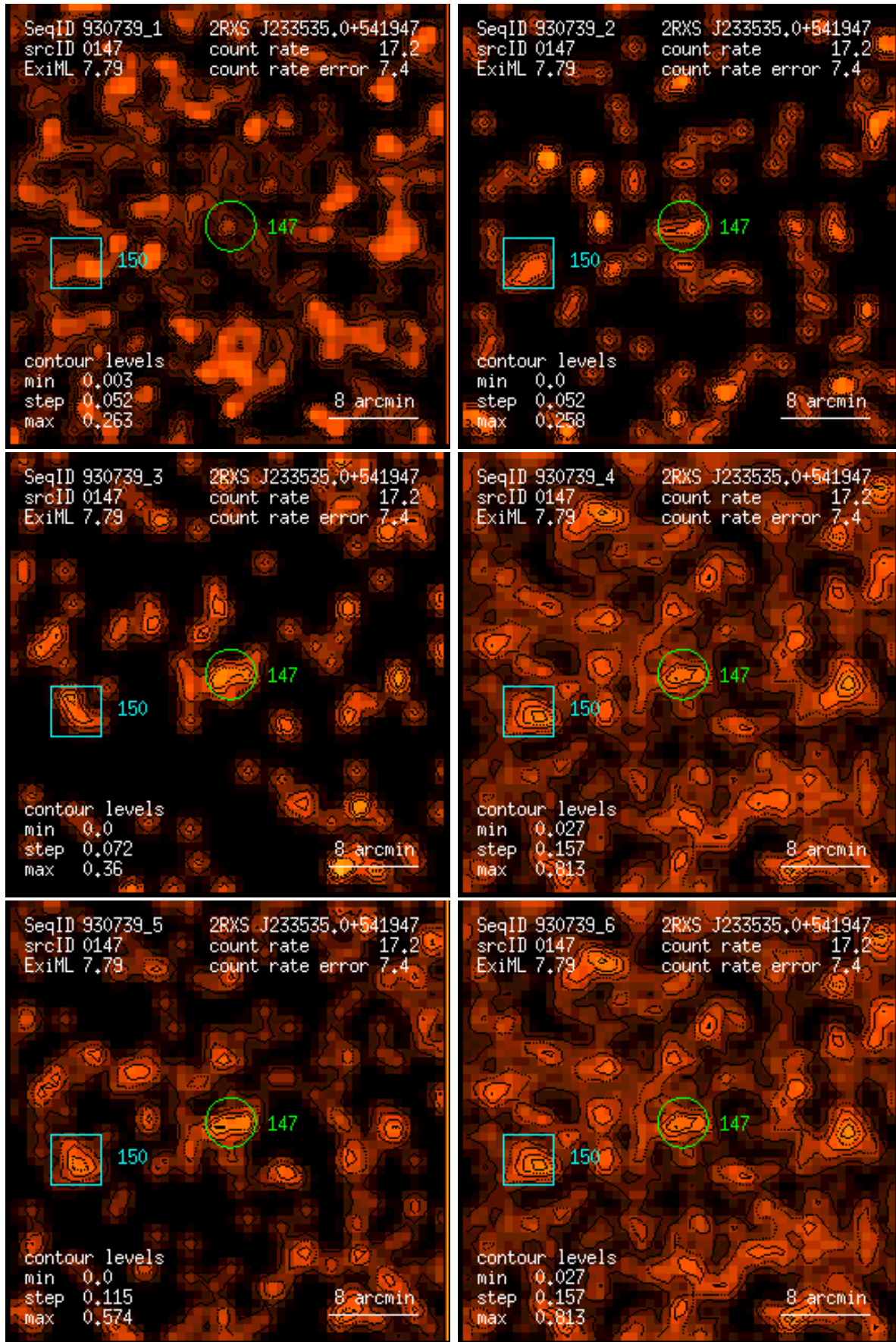
Figure 147: RASS 930739: detection 0147: band rate images, Gaussian filter: (1) PSPC channels 11 – 41, (2) 52 – 90, (3) 91 – 201, (4) 11 – 235, (5) 52 – 201, (6) 11 – 201. Broad band rates in counts/ks. Band rate contour levels in counts/ks/arcmin 2 .
