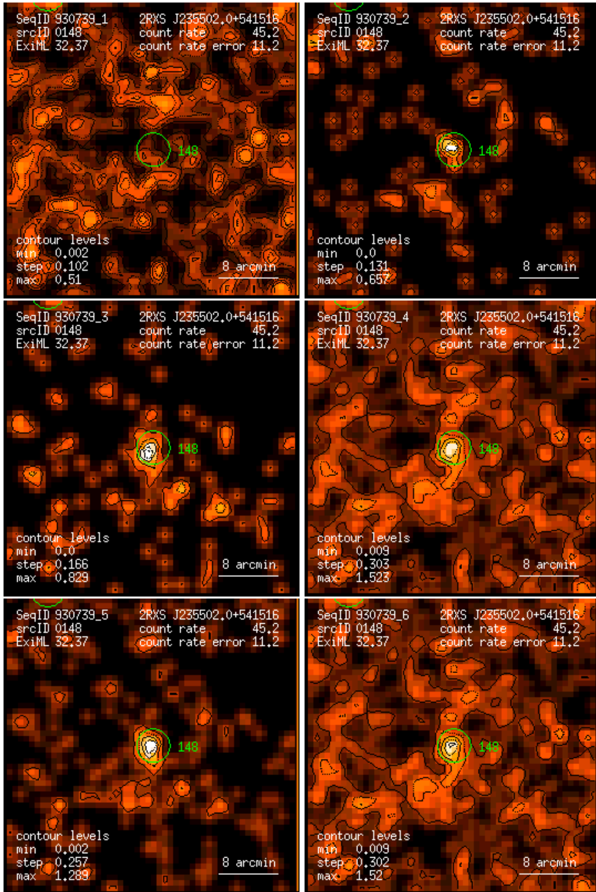
Figure 148: RASS 930739: detection 0148: band rate images, Gaussian filter: (1) PSPC channels 11 – 41, (2) 52 – 90, (3) 91 – 201, (4) 11 – 235, (5) 52 – 201, (6) 11 – 201. Broad band rates in counts/ks. Band rate contour levels in counts/ks/arcmin 2 .
