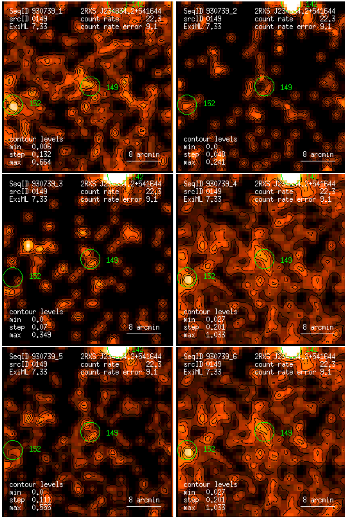
Figure 149: RASS 930739: detection 0149: band rate images, Gaussian filter: (1) PSPC channels 11 – 41, (2) 52 – 90, (3) 91 – 201, (4) 11 – 235, (5) 52 – 201, (6) 11 – 201. Broad band rates in counts/ks. Band rate contour levels in counts/ks/arcmin 2 .
