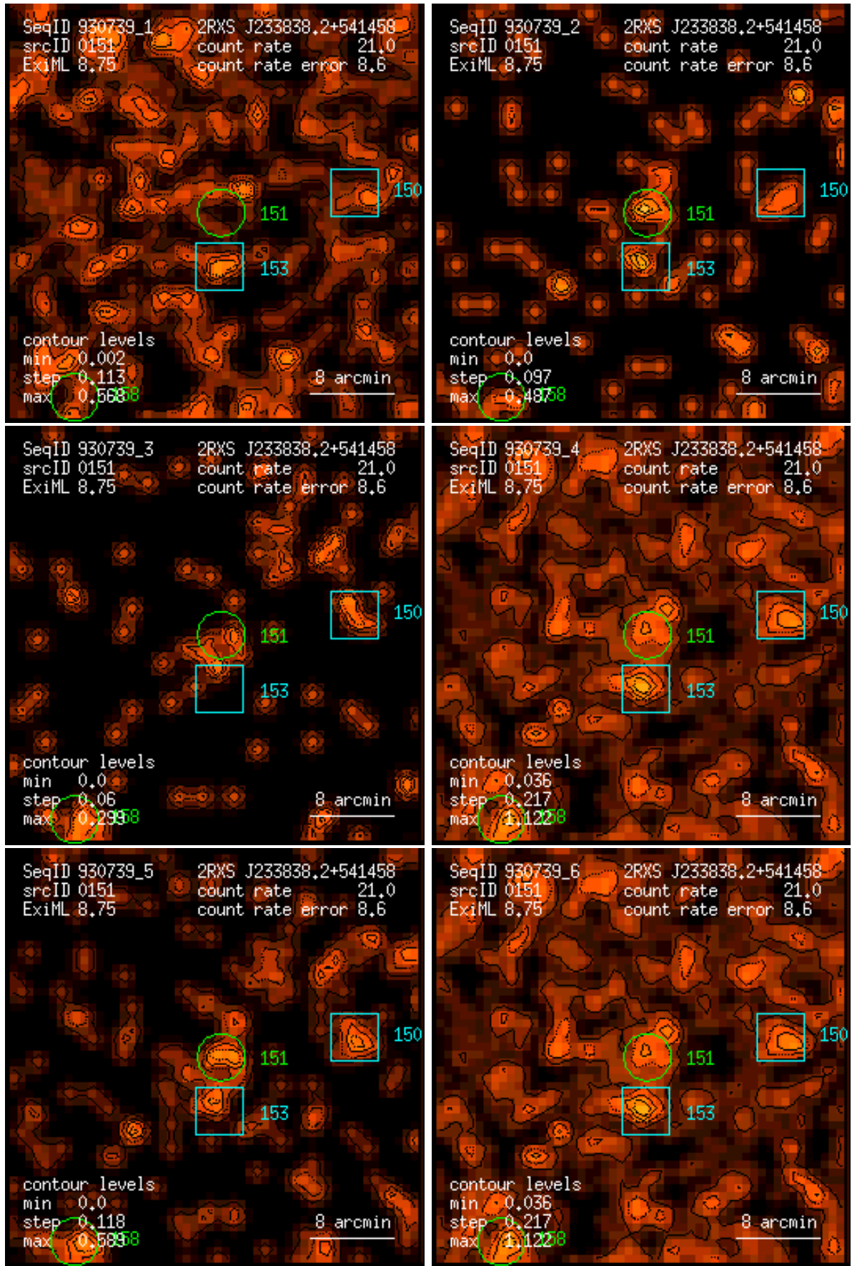
Figure 151: RASS 930739: detection 0151: band rate images, Gaussian filter: (1) PSPC channels 11 – 41, (2) 52 – 90, (3) 91 – 201, (4) 11 – 235, (5) 52 – 201, (6) 11 – 201. Broad band rates in counts/ks. Band rate contour levels in counts/ks/arcmin 2 .
