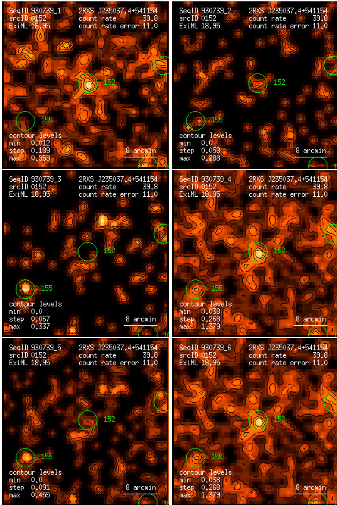
Figure 152: RASS 930739: detection 0152: band rate images, Gaussian filter: (1) PSPC channels 11 – 41, (2) 52 – 90, (3) 91 – 201, (4) 11 – 235, (5) 52 – 201, (6) 11 – 201. Broad band rates in counts/ks. Band rate contour levels in counts/ks/arcmin 2 .
