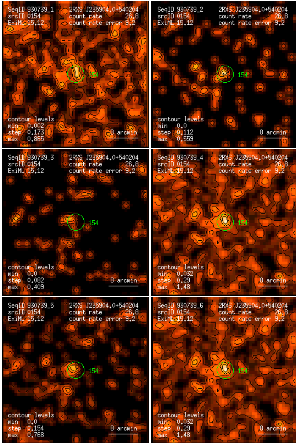
Figure 154: RASS 930739: detection 0154: band rate images, Gaussian filter: (1) PSPC channels 11 – 41, (2) 52 – 90, (3) 91 – 201, (4) 11 – 235, (5) 52 – 201, (6) 11 – 201. Broad band rates in counts/ks. Band rate contour levels in counts/ks/arcmin 2 .
