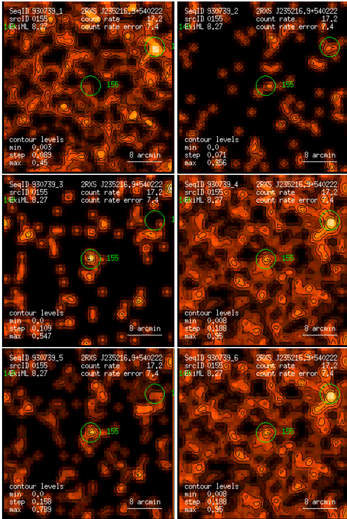
Figure 155: RASS 930739: detection 0155: band rate images, Gaussian filter: (1) PSPC channels 11 – 41, (2) 52 – 90, (3) 91 – 201, (4) 11 – 235, (5) 52 – 201, (6) 11 – 201. Broad band rates in counts/ks. Band rate contour levels in counts/ks/arcmin 2 .
