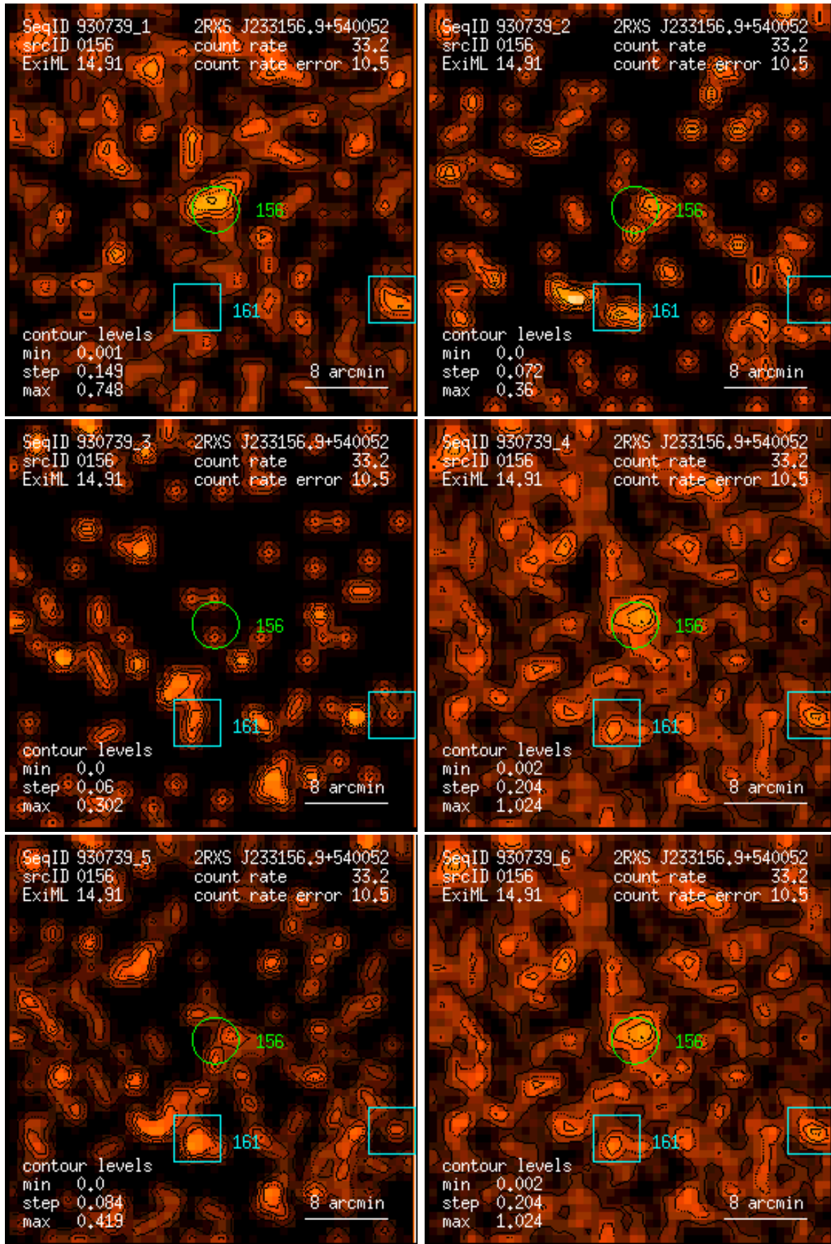
Figure 156: RASS 930739: detection 0156: band rate images, Gaussian filter: (1) PSPC channels 11 – 41, (2) 52 – 90, (3) 91 – 201, (4) 11 – 235, (5) 52 – 201, (6) 11 – 201. Broad band rates in counts/ks. Band rate contour levels in counts/ks/arcmin 2 .
