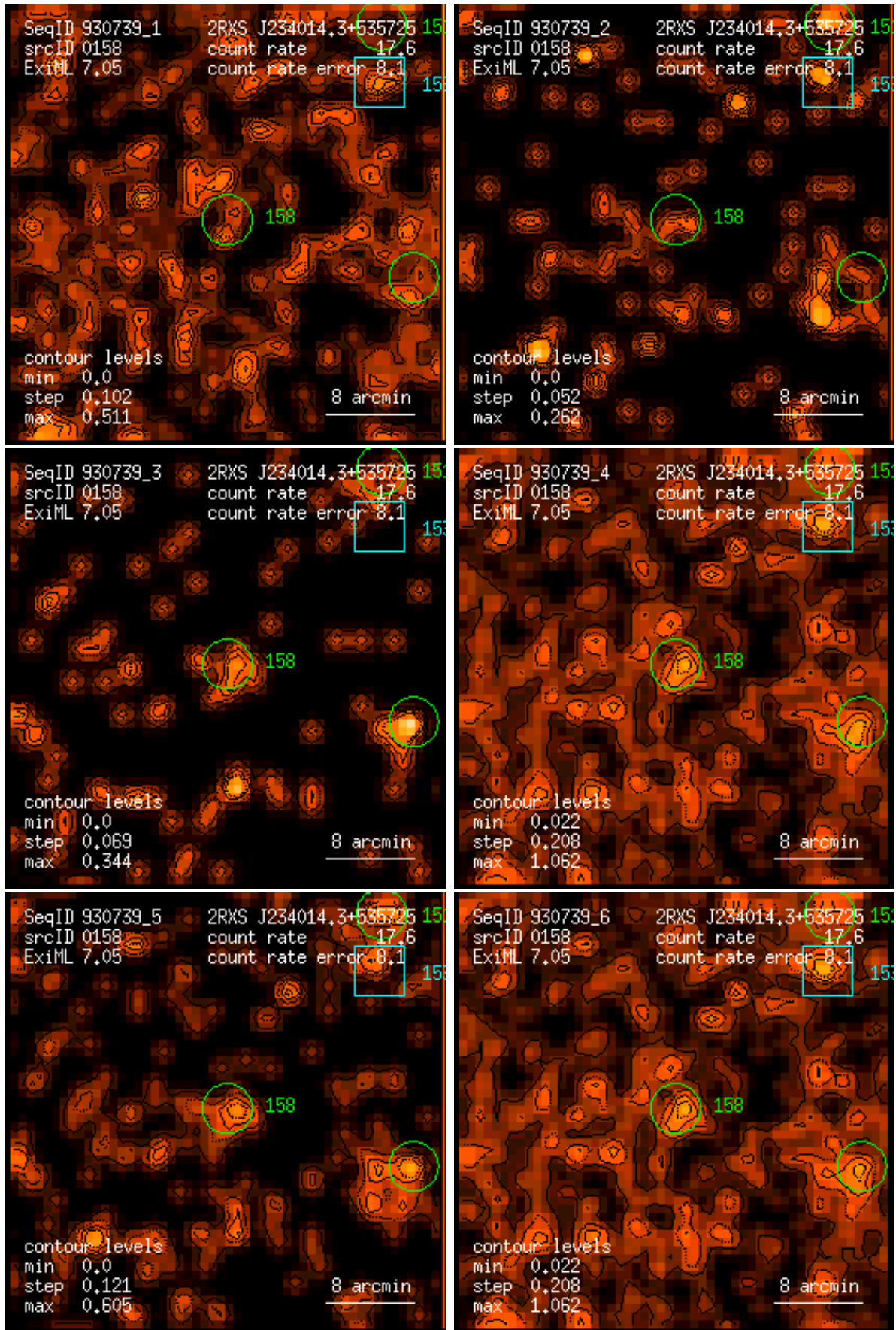
Figure 158: RASS 930739: detection 0158: band rate images, Gaussian filter: (1) PSPC channels 11 – 41, (2) 52 – 90, (3) 91 – 201, (4) 11 – 235, (5) 52 – 201, (6) 11 – 201. Broad band rates in counts/ks. Band rate contour levels in counts/ks/arcmin 2 .
