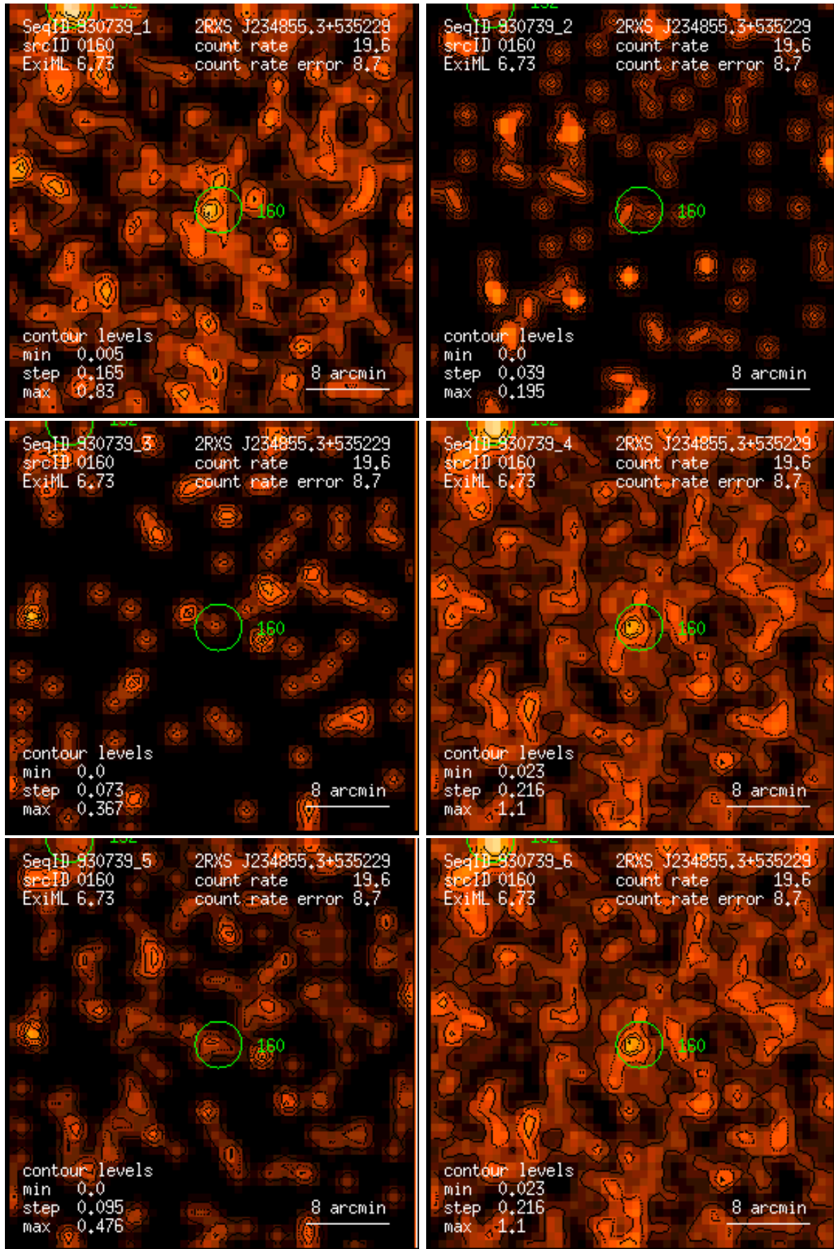
Figure 160: RASS 930739: detection 0160: band rate images, Gaussian filter: (1) PSPC channels 11 – 41, (2) 52 – 90, (3) 91 – 201, (4) 11 – 235, (5) 52 – 201, (6) 11 – 201. Broad band rates in counts/ks. Band rate contour levels in counts/ks/arcmin 2 .
