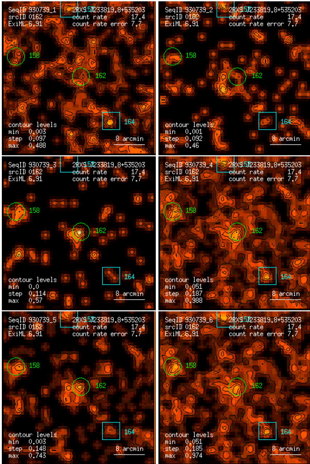
Figure 162: RASS 930739: detection 0162: band rate images, Gaussian filter: (1) PSPC channels 11 – 41, (2) 52 – 90, (3) 91 – 201, (4) 11 – 235, (5) 52 – 201, (6) 11 – 201. Broad band rates in counts/ks. Band rate contour levels in counts/ks/arcmin 2 .
