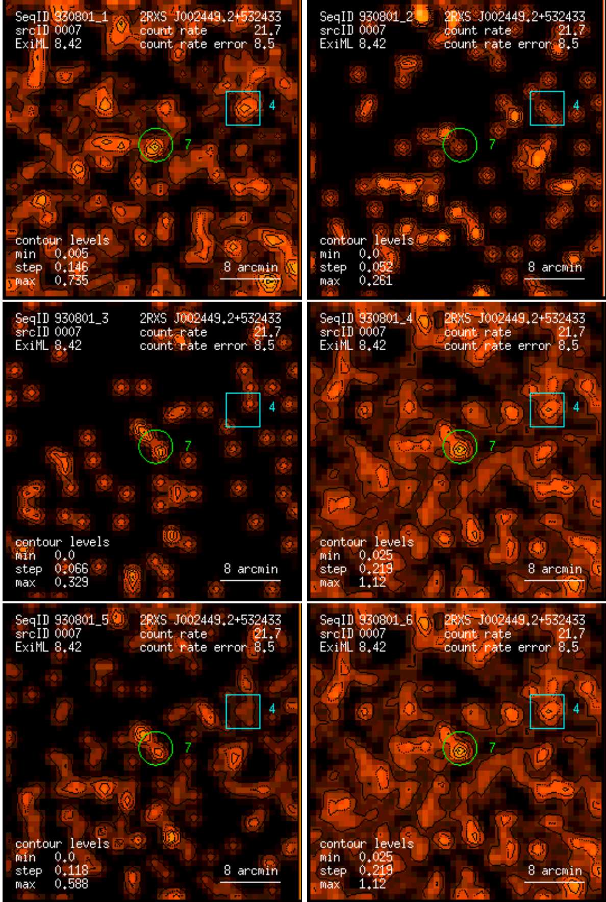
Figure 7: RASS 930801: detection 0007: band rate images, Gaussian filter: (1) PSPC channels 11 – 41, (2) 52 – 90, (3) 91 – 201, (4) 11 – 235, (5) 52 – 201, (6) 11 – 201. Broad band rates in counts/ks. Band rate contour levels in counts/ks/arcmin 2 .
