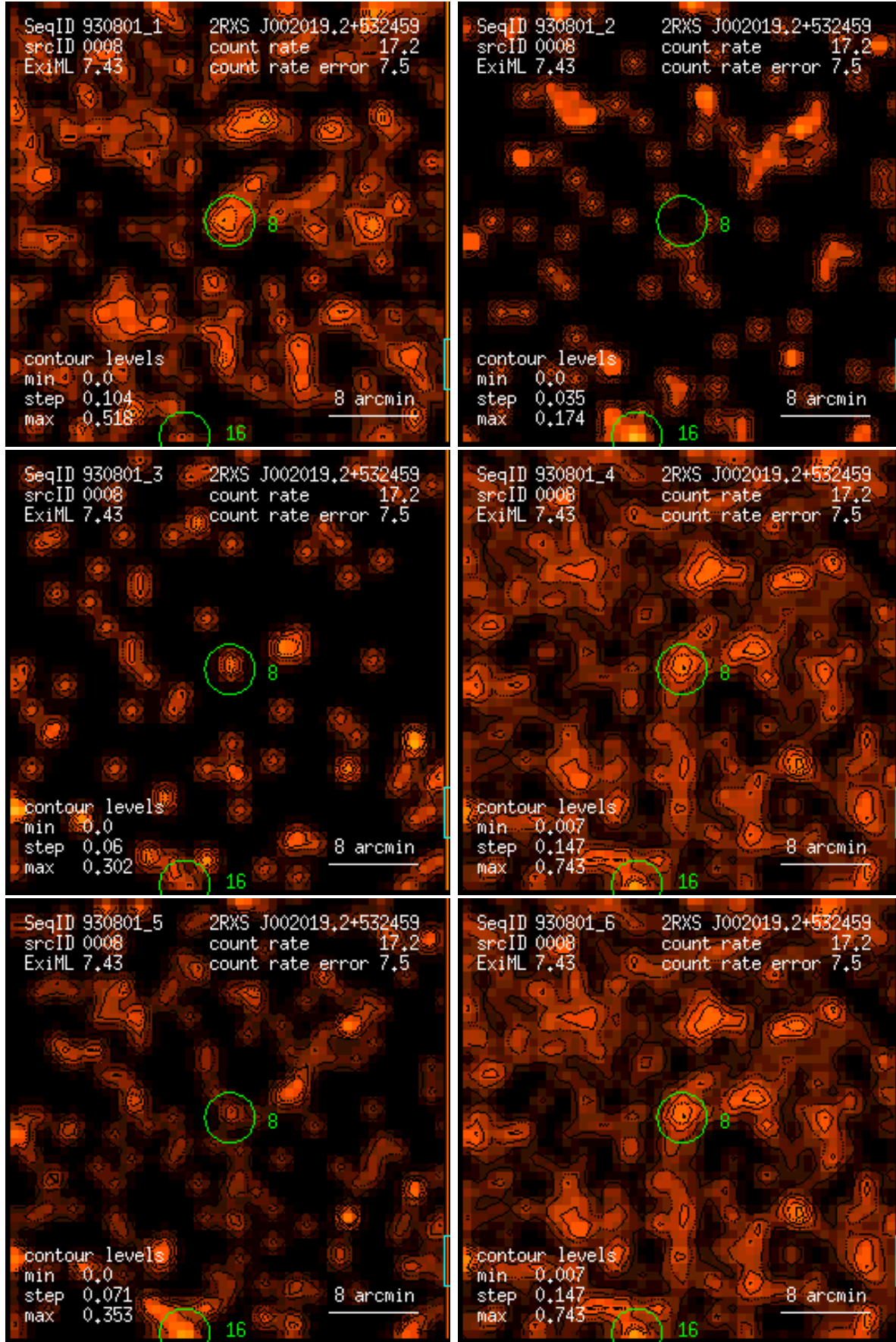
Figure 8: RASS 930801: detection 0008: band rate images, Gaussian filter: (1) PSPC channels 11 – 41, (2) 52 – 90, (3) 91 – 201, (4) 11 – 235, (5) 52 – 201, (6) 11 – 201. Broad band rates in counts/ks. Band rate contour levels in counts/ks/arcmin 2 .
