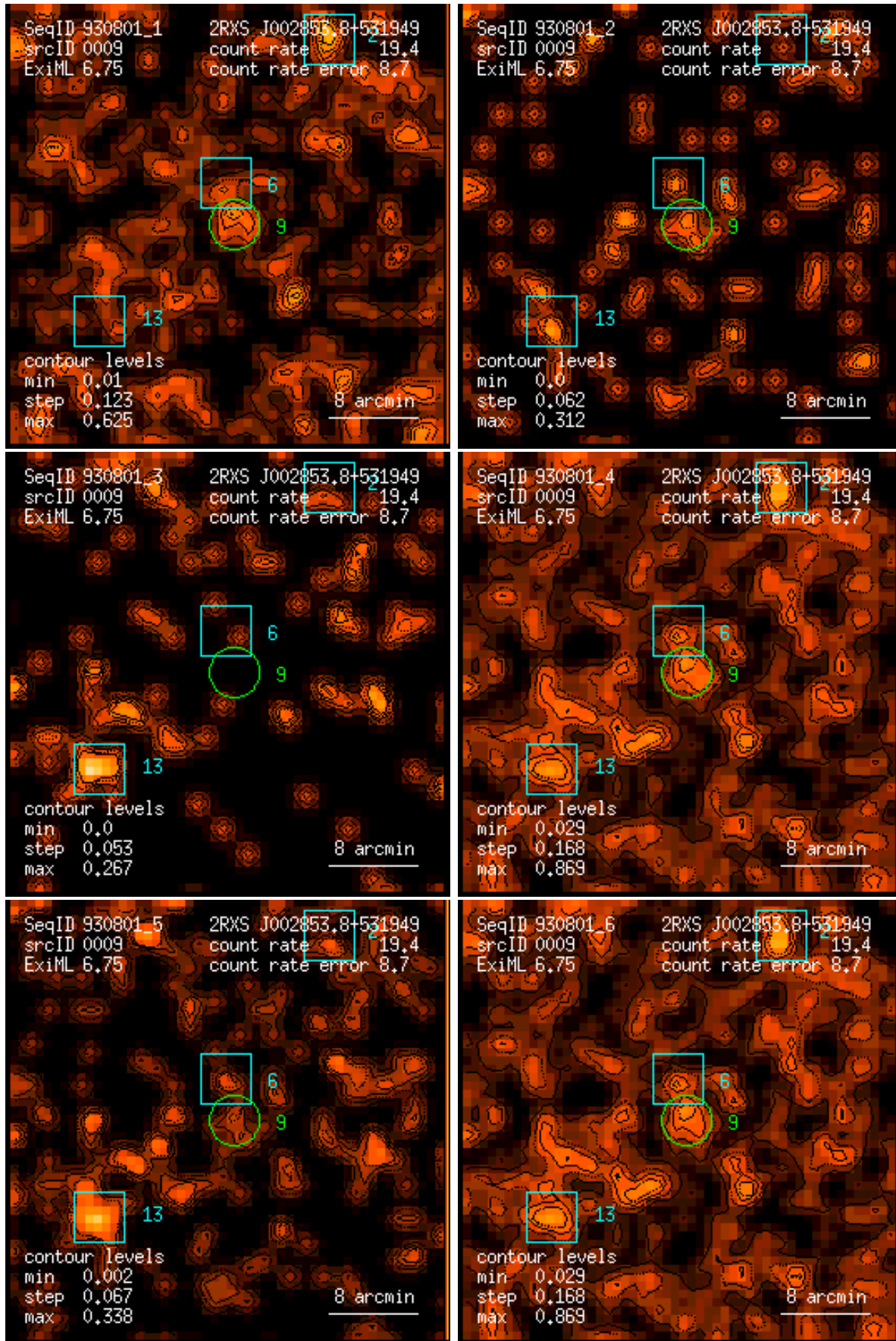
Figure 9: RASS 930801: detection 0009: band rate images, Gaussian filter: (1) PSPC channels 11 – 41, (2) 52 – 90, (3) 91 – 201, (4) 11 – 235, (5) 52 – 201, (6) 11 – 201. Broad band rates in counts/ks. Band rate contour levels in counts/ks/arcmin 2 .
