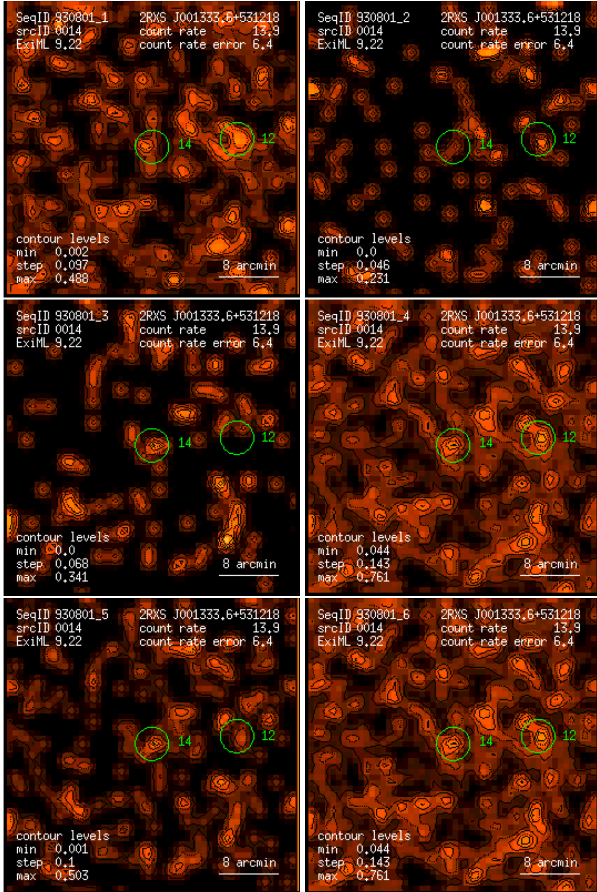
Figure 14: RASS 930801: detection 0014: band rate images, Gaussian filter: (1) PSPC channels 11 – 41, (2) 52 – 90, (3) 91 – 201, (4) 11 – 235, (5) 52 – 201, (6) 11 – 201. Broad band rates in counts/ks. Band rate contour levels in counts/ks/arcmin 2 .
