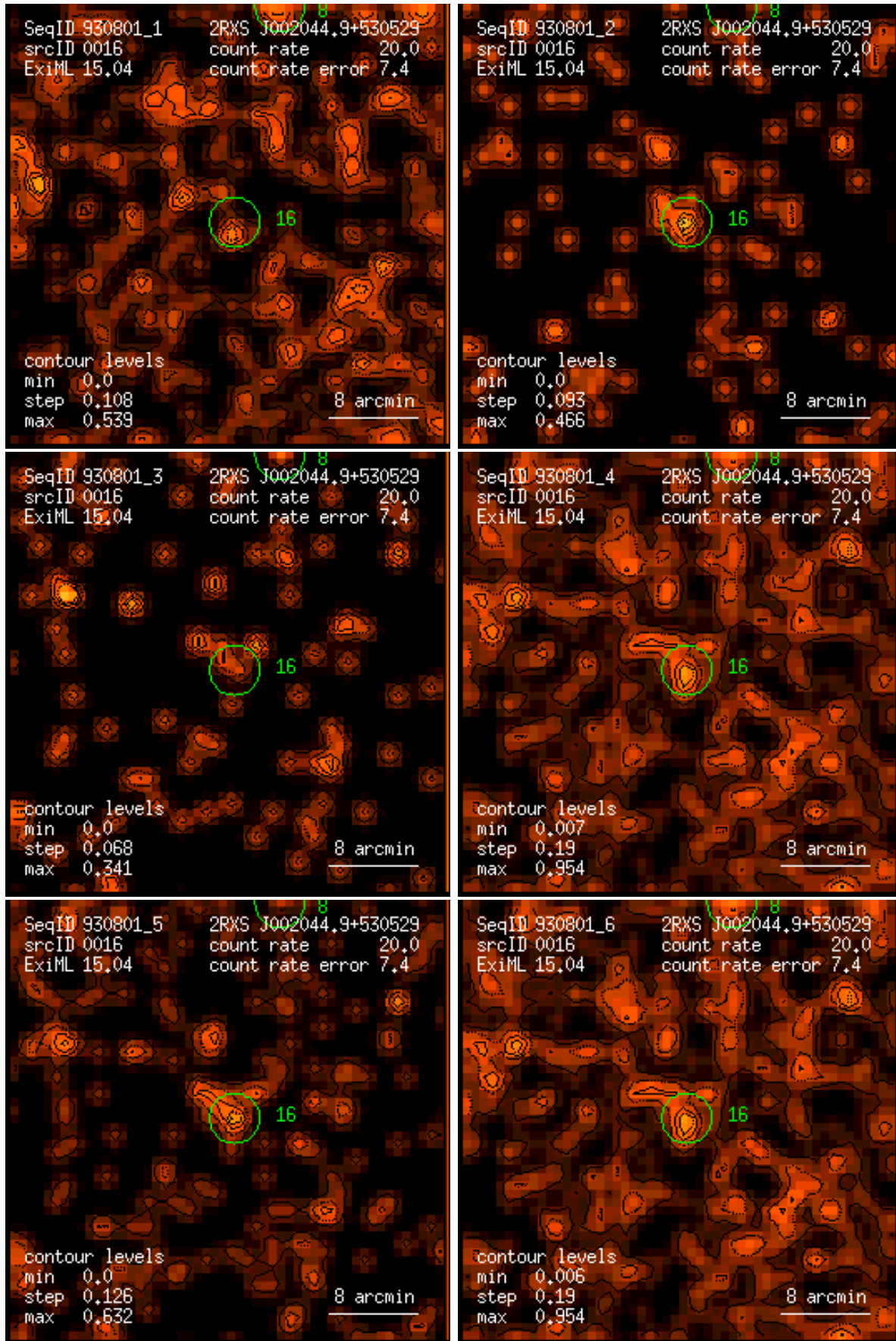
Figure 16: RASS 930801: detection 0016: band rate images, Gaussian filter: (1) PSPC channels 11 – 41, (2) 52 – 90, (3) 91 – 201, (4) 11 – 235, (5) 52 – 201, (6) 11 – 201. Broad band rates in counts/ks. Band rate contour levels in counts/ks/arcmin 2 .
