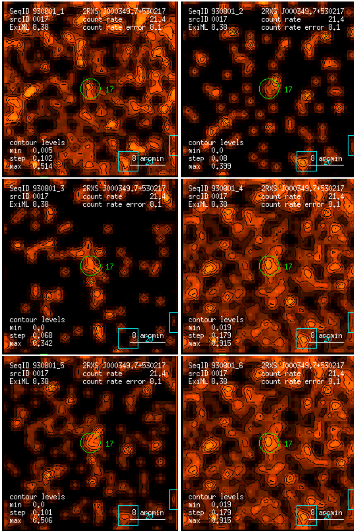
Figure 17: RASS 930801: detection 0017: band rate images, Gaussian filter: (1) PSPC channels 11 – 41, (2) 52 – 90, (3) 91 – 201, (4) 11 – 235, (5) 52 – 201, (6) 11 – 201. Broad band rates in counts/ks. Band rate contour levels in counts/ks/arcmin 2 .
