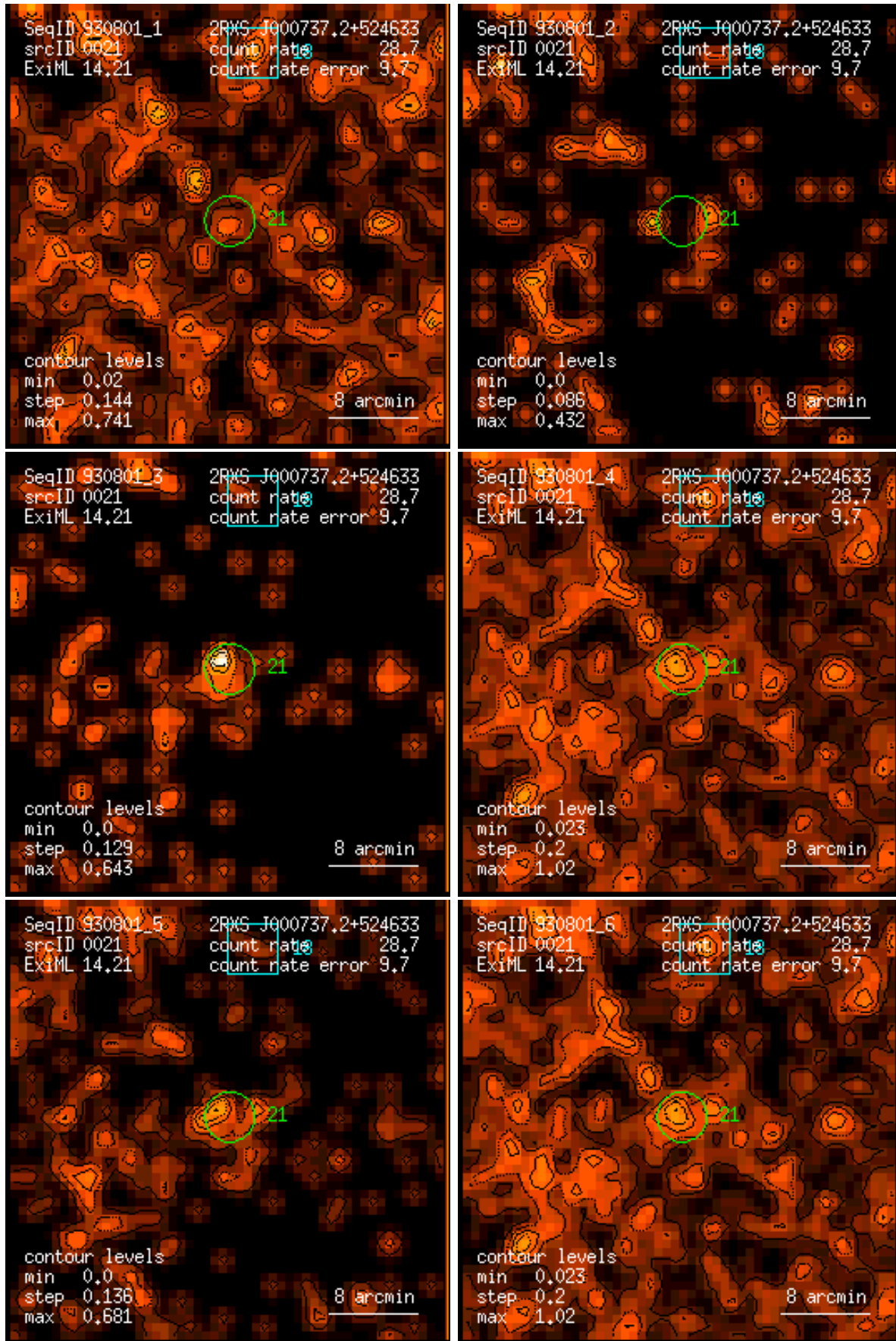
Figure 21: RASS 930801: detection 0021: band rate images, Gaussian filter: (1) PSPC channels 11 – 41, (2) 52 – 90, (3) 91 – 201, (4) 11 – 235, (5) 52 – 201, (6) 11 – 201. Broad band rates in counts/ks. Band rate contour levels in counts/ks/arcmin 2 .
