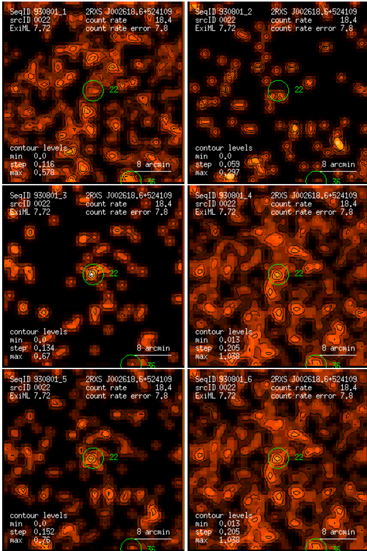
Figure 22: RASS 930801: detection 0022: band rate images, Gaussian filter: (1) PSPC channels 11 – 41, (2) 52 – 90, (3) 91 – 201, (4) 11 – 235, (5) 52 – 201, (6) 11 – 201. Broad band rates in counts/ks. Band rate contour levels in counts/ks/arcmin 2 .
