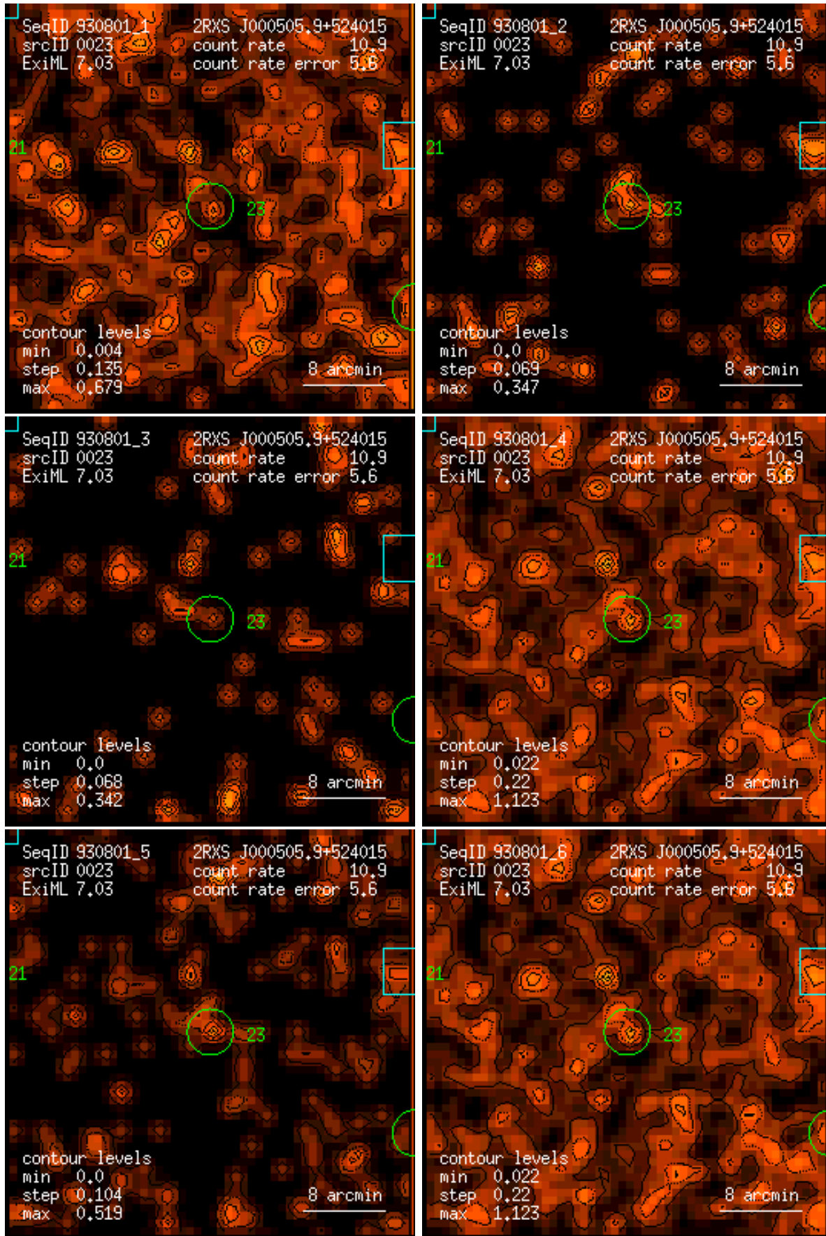
Figure 23: RASS 930801: detection 0023: band rate images, Gaussian filter: (1) PSPC channels 11 – 41, (2) 52 – 90, (3) 91 – 201, (4) 11 – 235, (5) 52 – 201, (6) 11 – 201. Broad band rates in counts/ks. Band rate contour levels in counts/ks/arcmin 2 .
