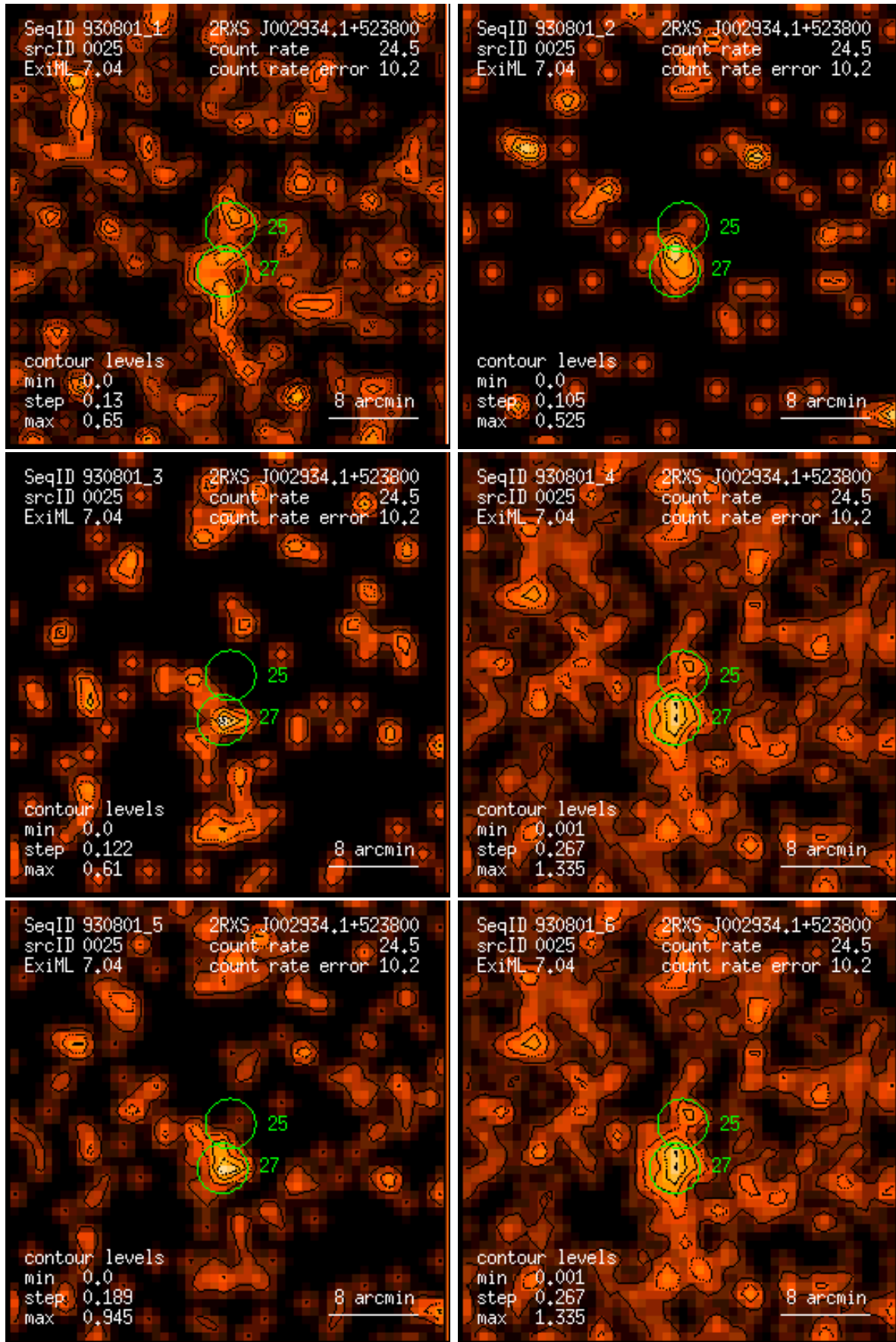
Figure 25: RASS 930801: detection 0025: band rate images, Gaussian filter: (1) PSPC channels 11 – 41, (2) 52 – 90, (3) 91 – 201, (4) 11 – 235, (5) 52 – 201, (6) 11 – 201. Broad band rates in counts/ks. Band rate contour levels in counts/ks/arcmin 2 .
